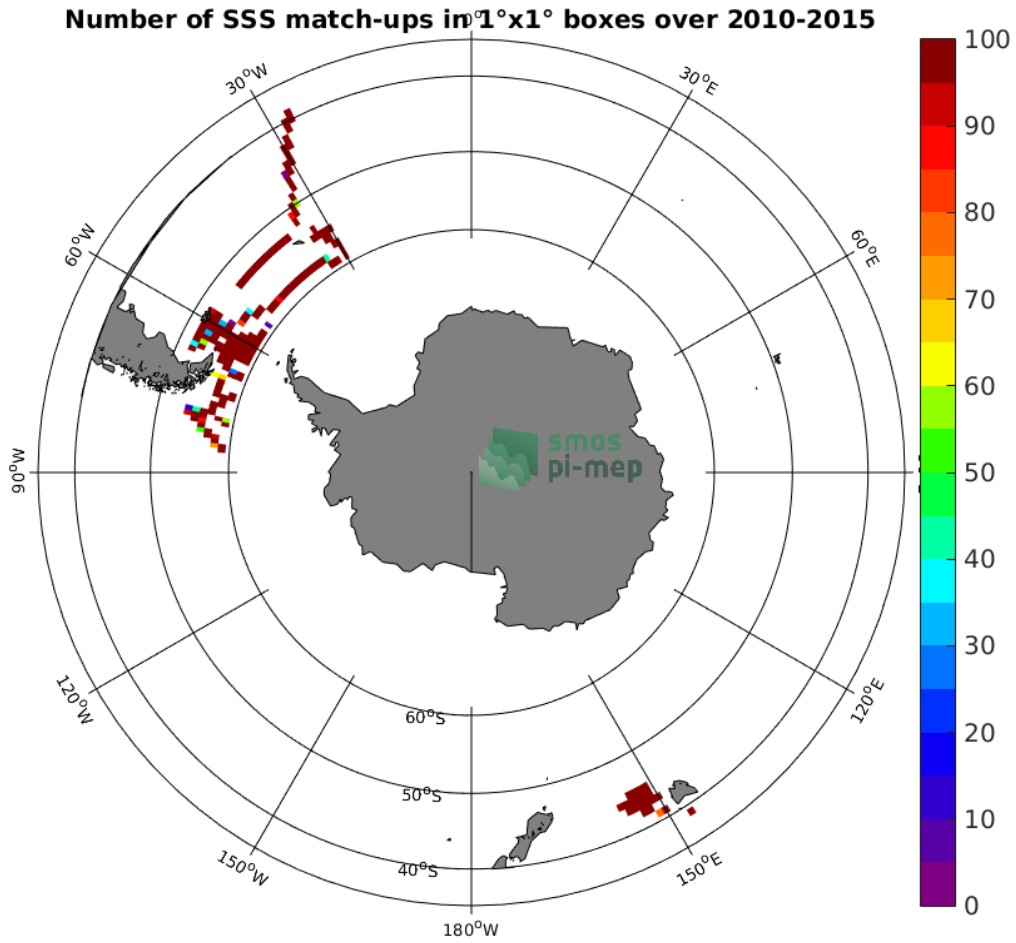
Figure 4: Number of SSS match-ups between TSG-SAMOS SSS and the SMOS L3 v2 - Daily - 0.5 Deg (CATDS-CECOS-IFREMER) SSS product for the Roaring Forties and Furious Fifties Pi-MEP region over 1°x1° boxes and for the full satellite product period.
