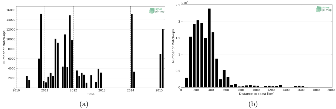
Figure 1: Number of match-ups between TSG-SAMOS and SMOS L3 v2 - Daily - 0.5 Deg (CATDS-CECOS-IFREMER) SSS as a function of time (a) and as function of the distance to coast (b) over the Roaring Forties and Furious Fifties Pi-MEP region and for the full satellite product period.
