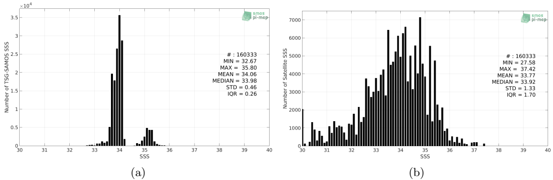
Figure 2: Histograms of SSS from TSG-SAMOS (a) and SMOS L3 v2 - Daily - 0.5 Deg (CATDS-CECOS-IFREMER) (b) considering all match-up pairs per bins of 0.1 over the Roaring Forties and Furious Fifties Pi-MEP region and for the full satellite product period.
