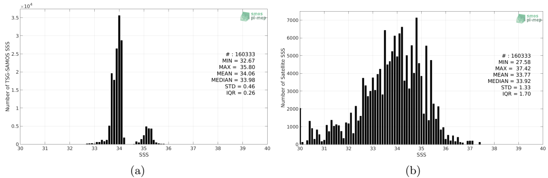
Figure 2: Histograms of SSS from TSG-SAMOS (a) and SMOS-L3-CATDS-CECOS-IFREMER-V2-1DAY-0.5DEG (b) considering all match-up pairs per bins of 0.1 over the Roaring Forties and Furious Fifties Pi-MEP region and for the full satellite product period.
