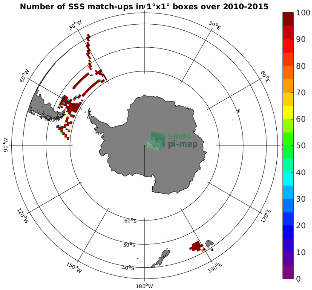
Figure 4: Number of SSS match-ups between TSG-SAMOS SSS and the SMOS-L3-CATDS-CECOS-IFREMER-V2-1DAY-0.5DEG SSS product for the Roaring Forties and Furious Fifties Pi-MEP region over 1^{\circ} \times 1^{\circ} boxes and for the full satellite product period.
