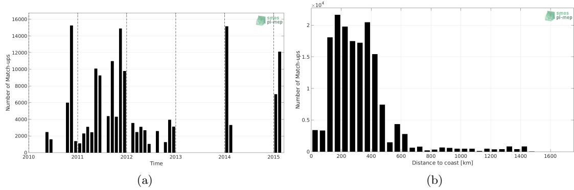
Figure 1: Number of match-ups between TSG-SAMOS and SMOS-L3-CATDS-CECOS-IFREMER-V2-1DAY-0.5DEG SSS as a function of time (a) and as function of the distance to coast (b) over the Roaring Forties and Furious Fifties Pi-MEP region and for the full satellite product period.
