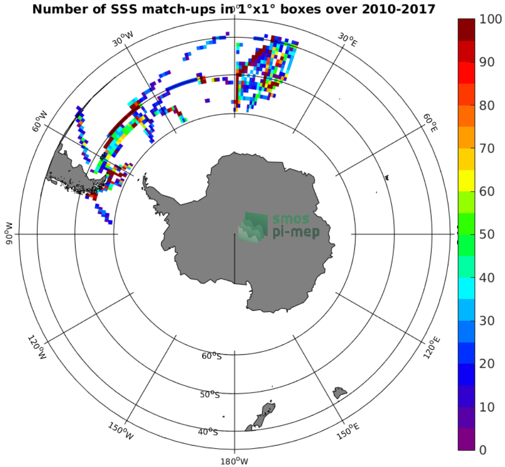
Figure 4: Number of SSS match-ups between TSG (Polarstern) SSS and the SMOS SSS L3 v2 - Daily - 0.5 Deg (CATDS-CECOS-IFREMER) SSS product for the Roaring Forties and Furious Fifties Pi-MEP region over 1°x1° boxes and for the full satellite product period.
