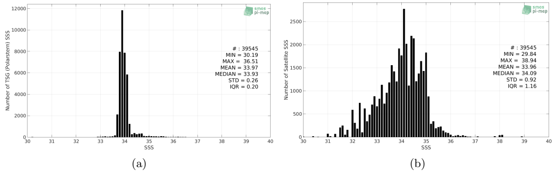
Figure 2: Histograms of SSS from TSG (Polarstern) (a) and SMOS SSS L3 v2 - Daily - 0.5 Deg (CATDS-CECOS-IFREMER) (b) considering all match-up pairs per bins of 0.1 over the Roaring Forties and Furious Fifties Pi-MEP region and for the full satellite product period.
