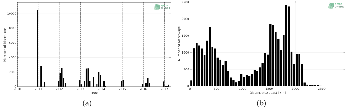
Figure 1: Number of match-ups between TSG (Polarstern) and SMOS SSS L3 v2 - Daily - 0.5 Deg (CATDS-CECOS-IFREMER) SSS as a function of time (a) and as function of the distance to coast (b) over the Roaring Forties and Furious Fifties Pi-MEP region and for the full satellite product period.
