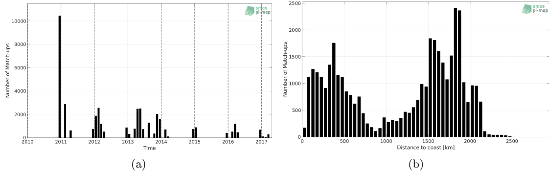
Figure 1: Number of match-ups between TSG-POLARSTERN and SMOS L3 v2 - Daily - 0.5 Deg (CATDS-CECOS-IFREMER) SSS as a function of time (a) and as function of the distance to coast (b) over the Roaring Forties and Furious Fifties Pi-MEP region and for the full satellite product period.
