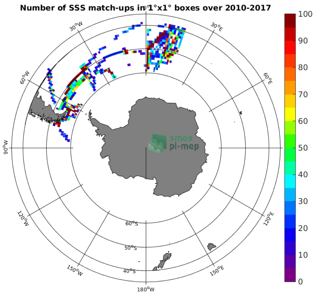
Figure 4: Number of SSS match-ups between TSG-POLARSTERN SSS and the SMOS-L3-CATDS-CECOS-IFREMER-V2-1DAY-0.5DEG SSS product for the Roaring Forties and Furious Fifties Pi-MEP region over 1°x1° boxes and for the full satellite product period.
