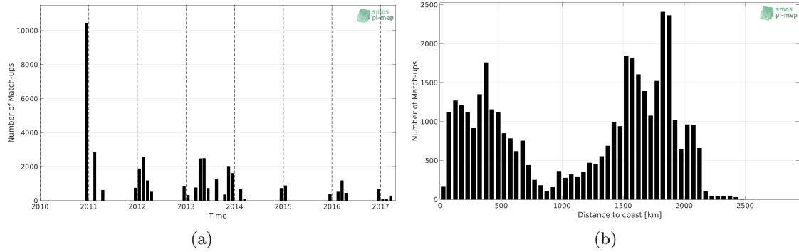
Figure 1: Number of match-ups between TSG-POLARSTERN and SMOS-L3-CATDS-CECOS-IFREMER-V2-1DAY-0.5DEG SSS as a function of time (a) and as function of the distance to coast (b) over the Roaring Forties and Furious Fifties Pi-MEP region and for the full satellite product period.
