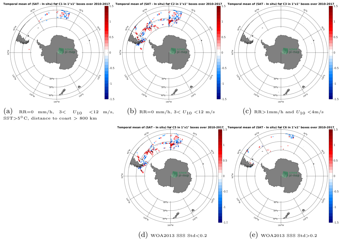
Figure 12: Temporal mean gridded over spatial boxes of size 1^\circ \times 1^\circ of \Delta SSS (SMOS-L3-CATDS-CECOS-IFREMER-V2-1DAY-0.5DEG - TSG-POLARSTERN) for 5 different subdatasets corresponding to: RR=0 mm/h, 3 < U_{10} < 12 m/s, SST >5^\circ\text{C} , distance to coast > 800 km (a), RR=0 mm/h, 3 < U_{10} < 12 m/s (b), RR >1 mm/h and U_{10} < 4 m/s (c), WOA2013 SSS Std <0.2 (d), WOA2013 SSS Std >0.2 (e).
