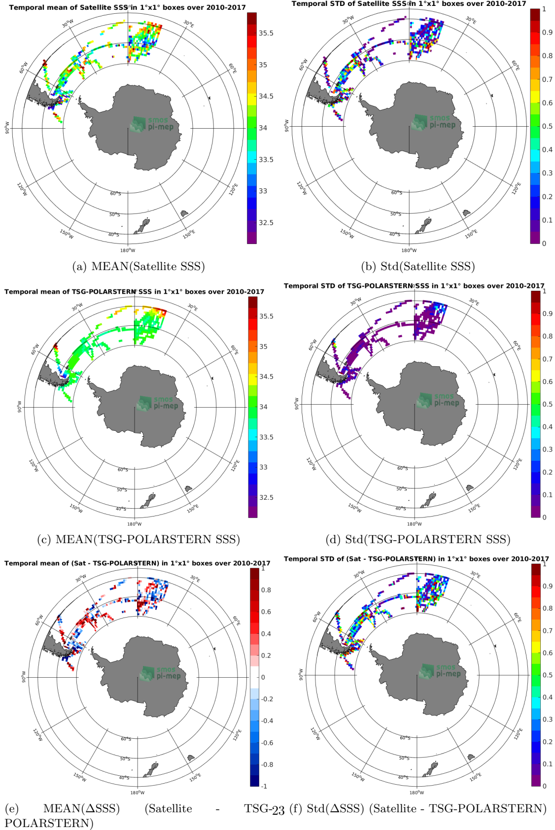
Figure 6: Temporal mean (left) and Std (right) of SSS from SMOS-L3-CATDS-CECOS-IFREMER-V2-1DAY-0.5DEG (top), TSG-POLARSTERN (middle), and of \Delta SSS (Satellite - TSG-POLARSTERN). Only match-up pairs are used to generate these maps.
