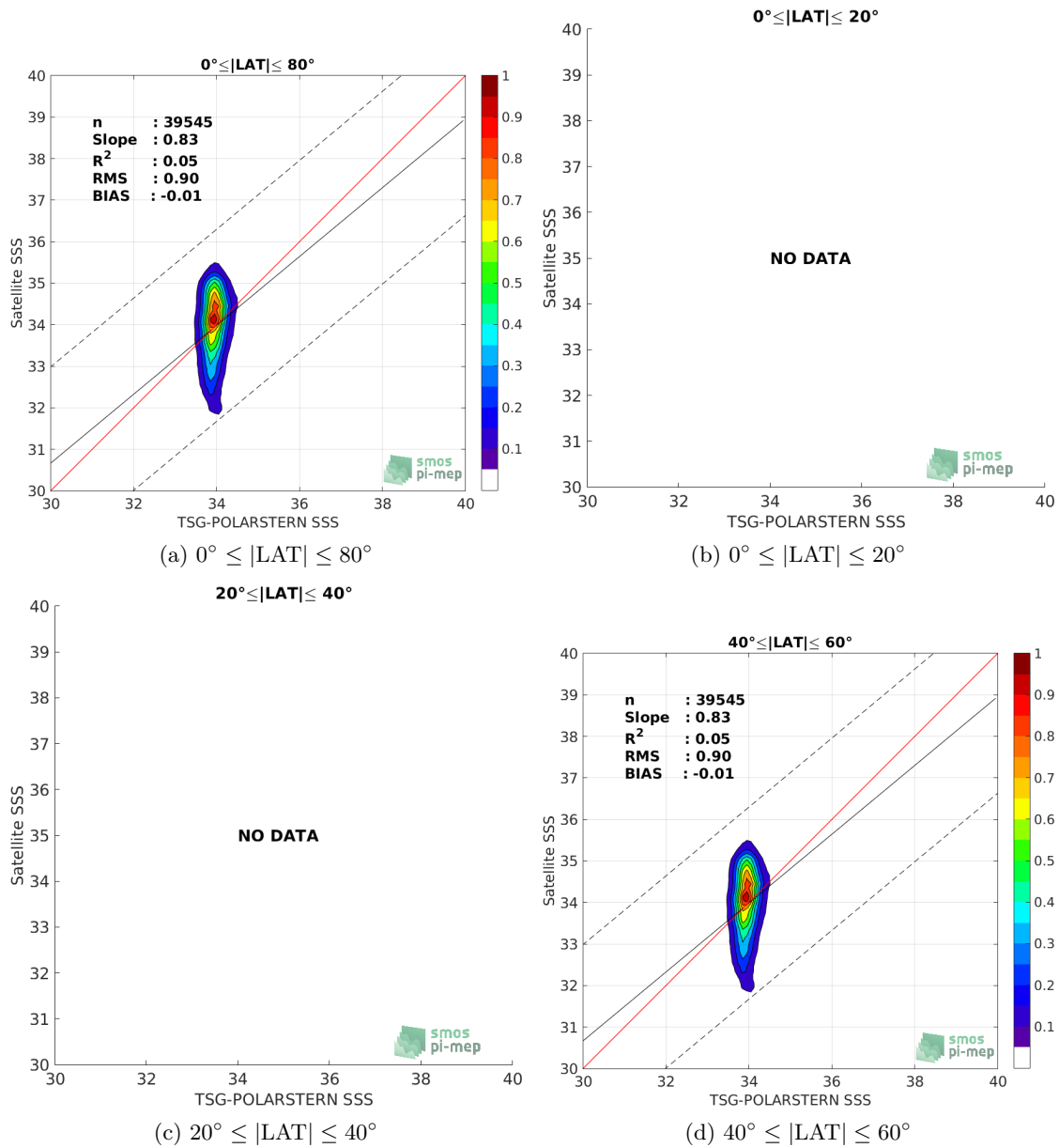
Figure 9: Contour maps of the concentration of SMOS-L3-CATDS-CECOS-IFREMER-V2-1DAY-0.5DEG SSS (y-axis) versus TSG-POLARSTERN SSS (x-axis) at match-up pairs for different latitude bands. For each plot, the red line shows x=y . The black thin and dashed lines indicate a linear fit through the data cloud and the \pm 95\% confidence levels, respectively. The number match-up pairs n , the slope and R^2 coefficient of the linear fit, the root mean square (RMS) and the mean bias between satellite and in situ data are indicated for each latitude band in each plots.
