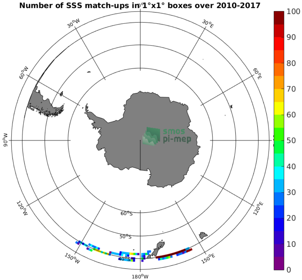
Figure 4: Number of SSS match-ups between TSG (LEGOS-DM) SSS and the SMOS SSS L3 v2 - Daily - 0.5 Deg (CATDS-CECOS-IFREMER) SSS product for the Roaring Forties and Furious Fifties Pi-MEP region over 1°x1° boxes and for the full satellite product period.
