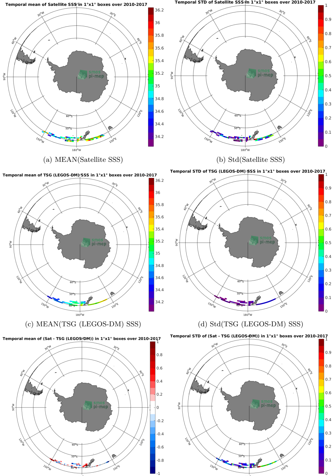
Figure 6: Temporal mean (left) and Std (right) of SSS from SMOS SSS L3 v2 - Daily - 0.5 Deg (CATDS-CECOS-IFREMER) (top), TSG (LEGOS-DM) (middle), and of \Delta SSS (Satellite - TSG (LEGOS-DM)). Only match-up pairs are used to generate these maps.
