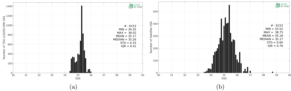
Figure 2: Histograms of SSS from TSG (LEGOS-DM) (a) and SMOS SSS L3 v2 - Daily - 0.5 Deg (CATDS-CECOS-IFREMER) (b) considering all match-up pairs per bins of 0.1 over the Roaring Forties and Furious Fifties Pi-MEP region and for the full satellite product period.
