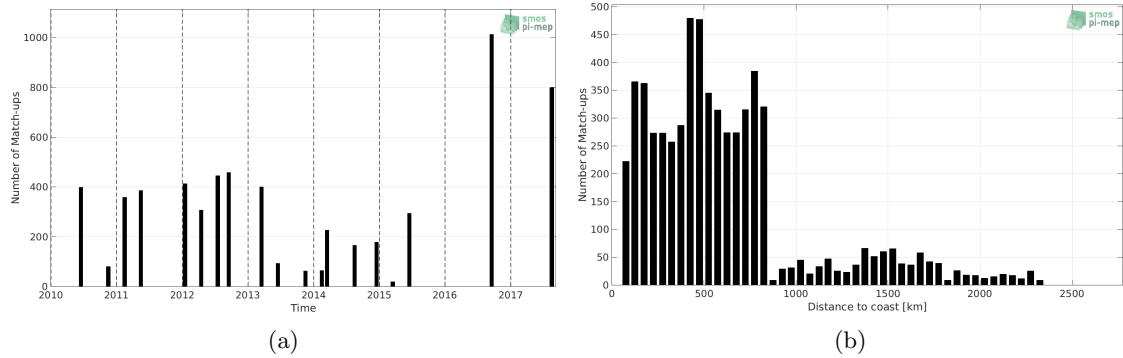
Figure 1: Number of match-ups between TSG (LEGOS-DM) and SMOS SSS L3 v2 - Daily - 0.5 Deg (CATDS-CECOS-IFREMER) SSS as a function of time (a) and as function of the distance to coast (b) over the Roaring Forties and Furious Fifties Pi-MEP region and for the full satellite product period.
