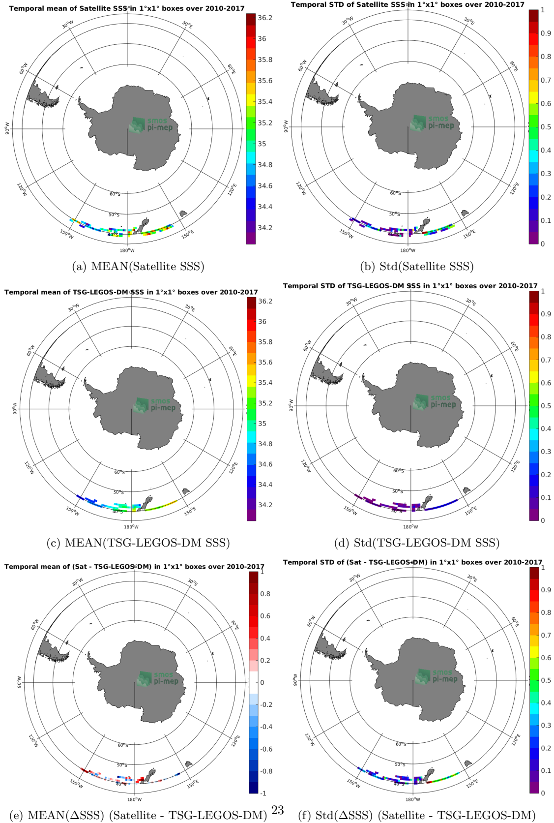
Figure 6: Temporal mean (left) and Std (right) of SSS from SMOS-L3-CATDS-CECOS-IFREMER-V2-1DAY-0.5DEG (top), TSG-LEGOS-DM (middle), and of \Delta SSS (Satellite - TSG-LEGOS-DM). Only match-up pairs are used to generate these maps.
