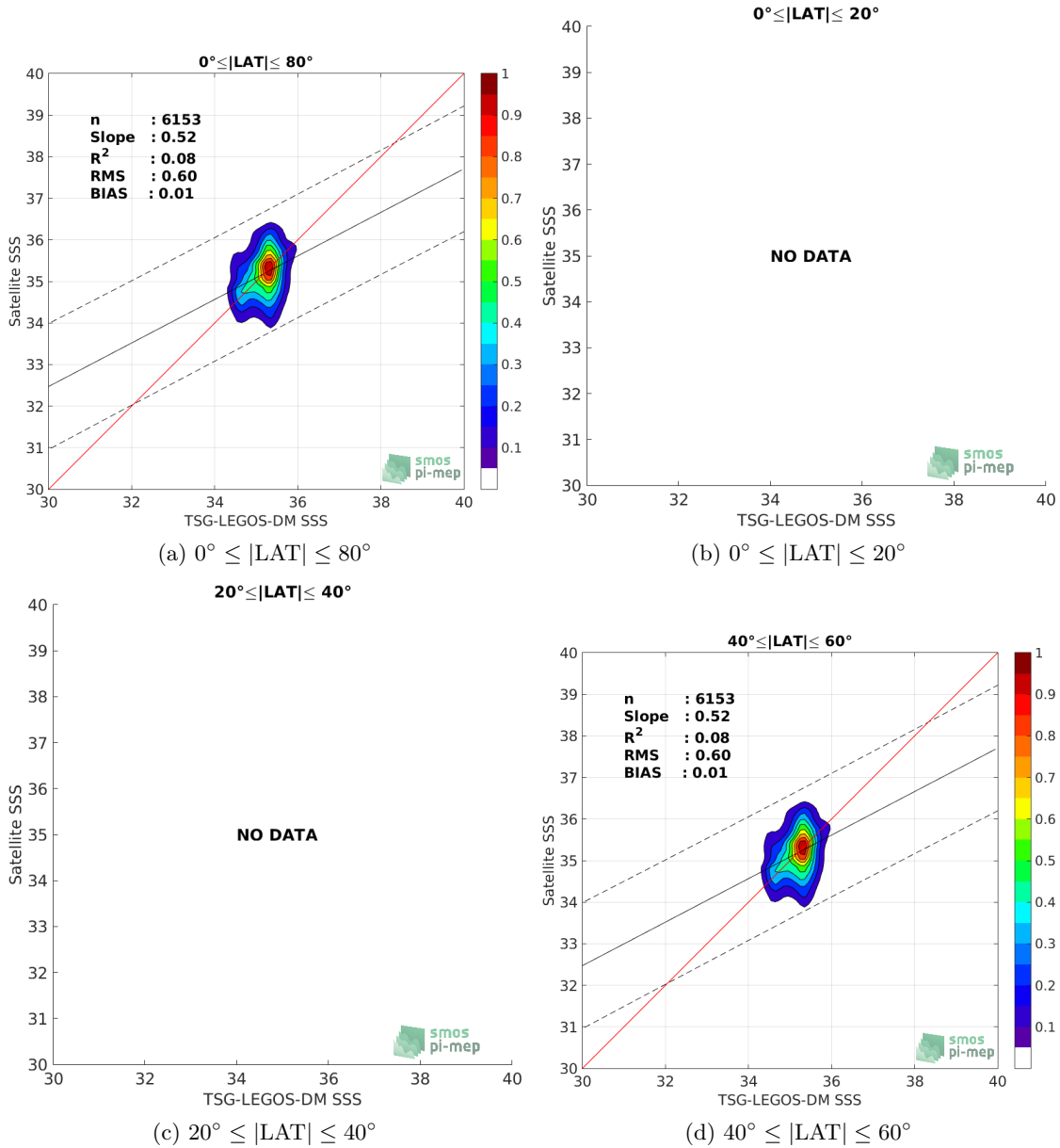
Figure 9: Contour maps of the concentration of SMOS-L3-CATDS-CECOS-IFREMER-V2-1DAY-0.5DEG SSS (y-axis) versus TSG-LEGOS-DM SSS (x-axis) at match-up pairs for different latitude bands. For each plot, the red line shows x=y . The black thin and dashed lines indicate a linear fit through the data cloud and the \pm 95\% confidence levels, respectively. The number match-up pairs n , the slope and R^2 coefficient of the linear fit, the root mean square (RMS) and the mean bias between satellite and in situ data are indicated for each latitude band in each plots.
