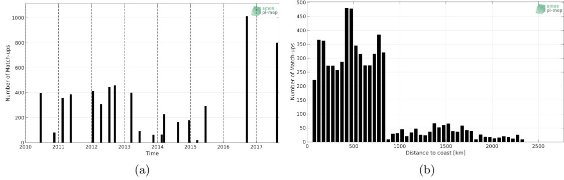
Figure 1: Number of match-ups between TSG-LEGOS-DM and SMOS-L3-CATDS-CECOS-IFREMER-V2-1DAY-0.5DEG SSS as a function of time (a) and as function of the distance to coast (b) over the Roaring Forties and Furious Fifties Pi-MEP region and for the full satellite product period.
