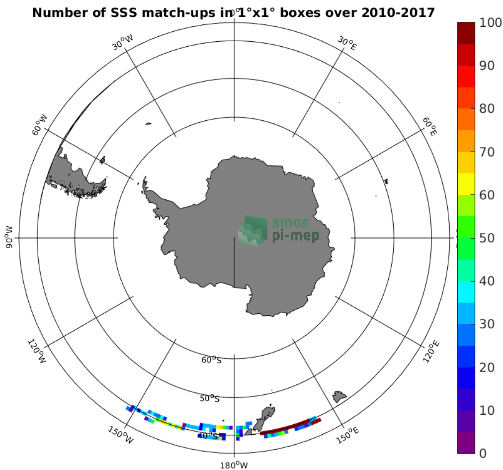
Figure 4: Number of SSS match-ups between TSG-LEGOS-DM SSS and the SMOS-L3-CATDS-CECOS-IFREMER-V2-1DAY-0.5DEG SSS product for the Roaring Forties and Furious Fifties Pi-MEP region over 1°x1° boxes and for the full satellite product period.
