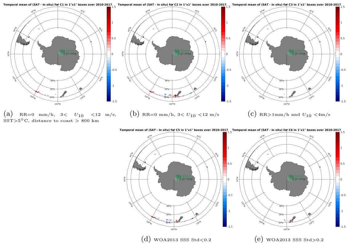
Figure 12: Temporal mean gridded over spatial boxes of size 1^\circ \times 1^\circ of \Delta SSS (SMOS-L3-CATDS-CECOS-IFREMER-V2-1DAY-0.5DEG - TSG-LEGOS-DM) for 5 different subdatasets corresponding to:RR=0 mm/h, 3 < U_{10} < 12 m/s, SST >5^\circ C, distance to coast > 800 km (a), RR=0 mm/h, 3 < U_{10} < 12 m/s (b), RR >1 mm/h and U_{10} < 4 m/s (c), WOA2013 SSS Std <0.2 (d), WOA2013 SSS Std >0.2 (e).
