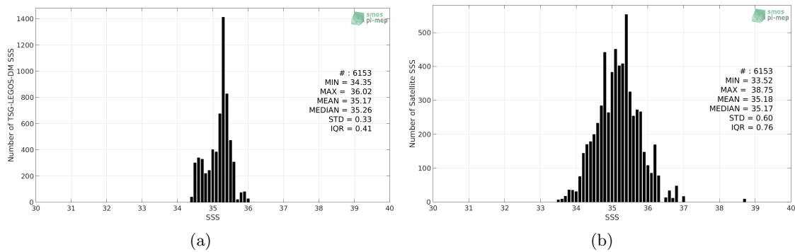
Figure 2: Histograms of SSS from TSG-LEGOS-DM (a) and SMOS-L3-CATDS-CECOS-IFREMER-V2-1DAY-0.5DEG (b) considering all match-up pairs per bins of 0.1 over the Roaring Forties and Furious Fifties Pi-MEP region and for the full satellite product period.
