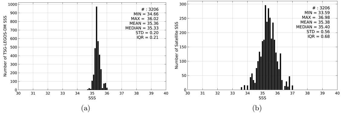
Figure 2: Histograms of SSS from TSG-LEGOS-DM (a) and SMOS-L3-CATDS-CECOS-IFREMER-V2-1DAY-0.5deg (b) considering all match-up pairs per bins of 0.1 over the Roaring Forties and Furious Fifties Pi-MEP region and for the full satellite product period.
