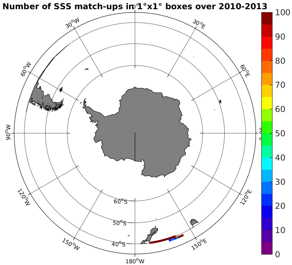
Figure 4: Number of SSS match-ups between TSG-LEGOS-DM SSS and the SMOS-L3-CATDS-CECOS-IFREMER-V2-1DAY-0.5deg SSS product for the Roaring Forties and Furious Fifties Pi-MEP region over 1°x1° boxes and for the full satellite product period.
