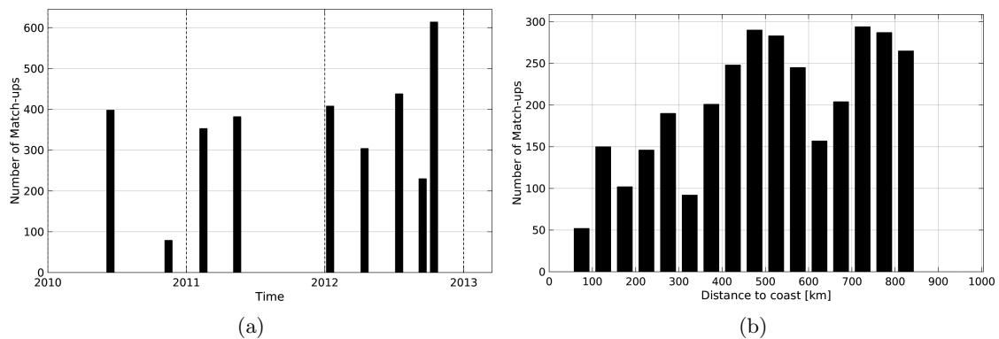
Figure 1: Number of match-ups between TSG-LEGOS-DM and SMOS-L3-CATDS-CECOS-IFREMER-V2-1DAY-0.5deg SSS as a function of time (a) and as function of the distance to coast (b) over the Roaring Forties and Furious Fifties Pi-MEP region and for the full satellite product period.
