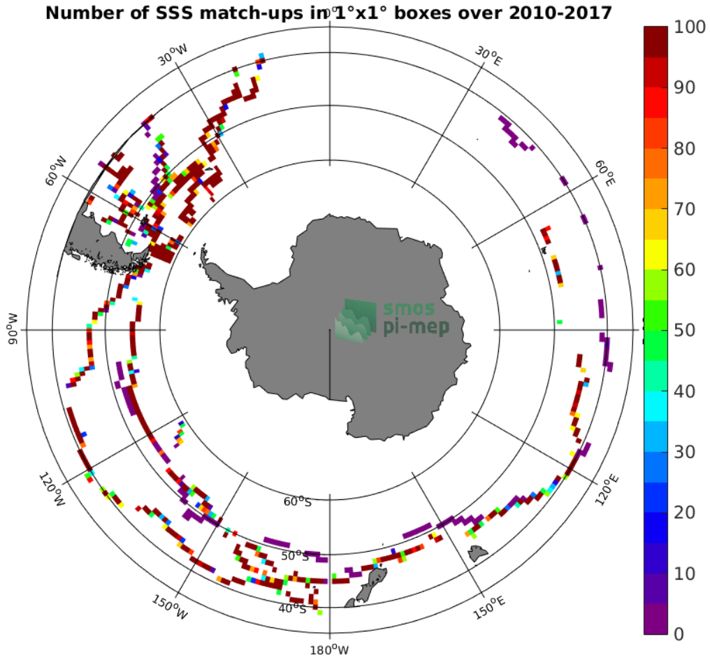
Figure 4: Number of SSS match-ups between TSG (GOSUD-Sailing-ship) SSS and the SMOS SSS L3 v2 - Daily - 0.5 Deg (CATDS-CECOS-IFREMER) SSS product for the Roaring Forties and Furious Fifties Pi-MEP region over 1^\circ \times 1^\circ boxes and for the full satellite product period.
