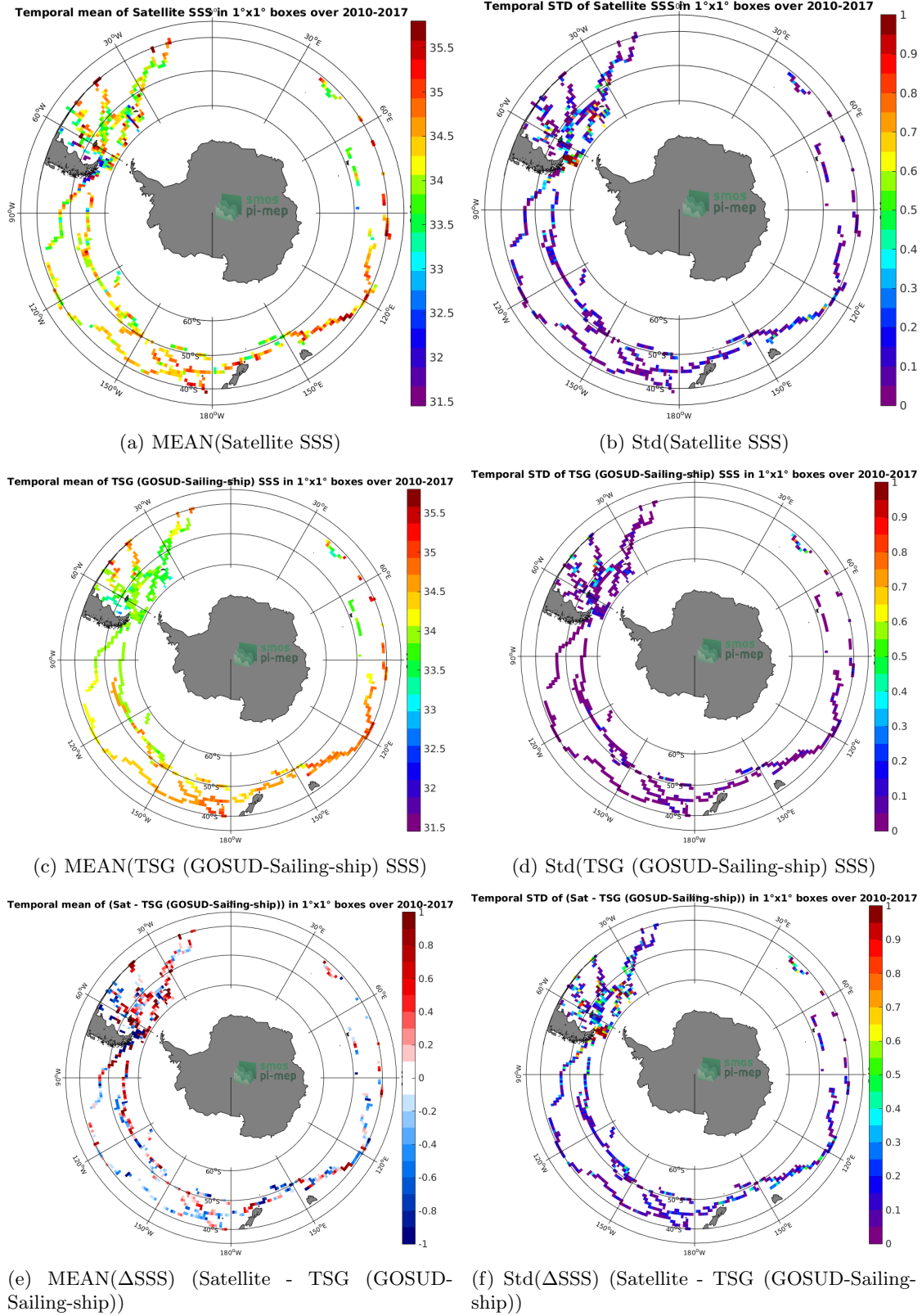
Figure 6: Temporal mean (left) and Std (right) of SSS from SMOS SSS L3 v2 - Daily - 0.5 Deg (CATDS-CECOS-IFREMER) (top), TSG 0 (GOSUD-Sailing-ship) (middle), and of \Delta SSS (Satellite - TSG (GOSUD-Sailing-ship)). Only match-up pairs are used to generate these maps.
