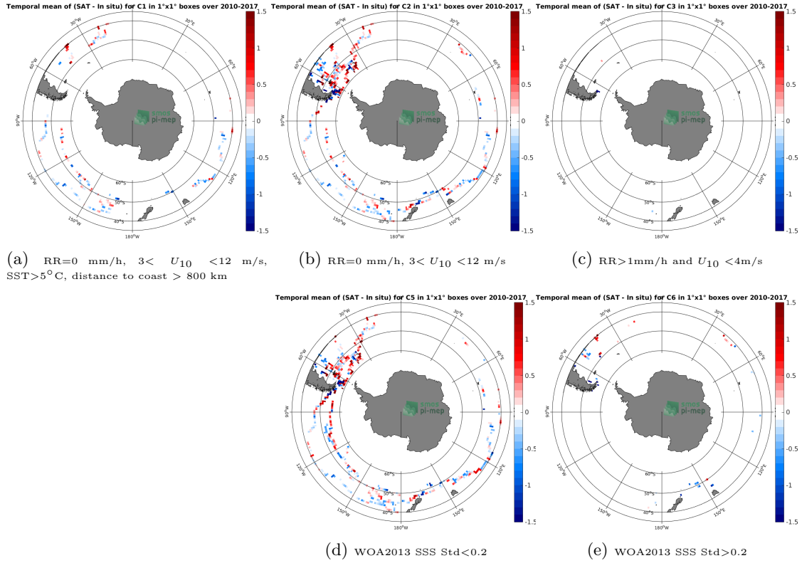
Figure 12: Temporal mean gridded over spatial boxes of size 1°x1° of \Delta SSS (SMOS SSS L3 v2 - Daily - 0.5 Deg (CATDS-CECOS-IFREMER) - TSG (GOSUD-Sailing-ship)) for 5 different subdatasets corresponding to:RR=0 mm/h, 3 < U_{10} < 12 m/s, SST>5°C, distance to coast > 800 km (a), RR=0 mm/h, 3 < U_{10} < 12 m/s (b), RR>1mm/h and U_{10} < 4 m/s (c), WOA2013 SSS Std<0.2 (d), WOA2013 SSS Std>0.2 (e).
