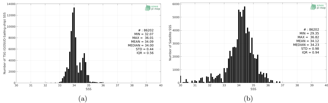
Figure 2: Histograms of SSS from TSG (GOSUD-Sailing-ship) (a) and SMOS SSS L3 v2 - Daily - 0.5 Deg (CATDS-CECOS-IFREMER) (b) considering all match-up pairs per bins of 0.1 over the Roaring Forties and Furious Fifties Pi-MEP region and for the full satellite product period.
