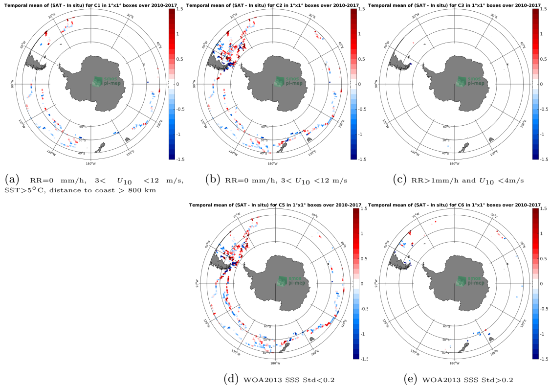
Figure 12: Temporal mean gridded over spatial boxes of size 1°x1° of \Delta SSS (SMOS L3 v2 - Daily - 0.5 Deg (CATDS-CECOS-IFREMER) - TSG-GOSUD-Sailing-ship) for 5 different subdatasets corresponding to:RR=0 mm/h, 3 < U_{10} < 12 m/s, SST>5°C, distance to coast > 800 km (a), RR=0 mm/h, 3 < U_{10} < 12 m/s (b), RR>1mm/h and U_{10} < 4 m/s (c), WOA2013 SSS Std<0.2 (d), WOA2013 SSS Std>0.2 (e).
