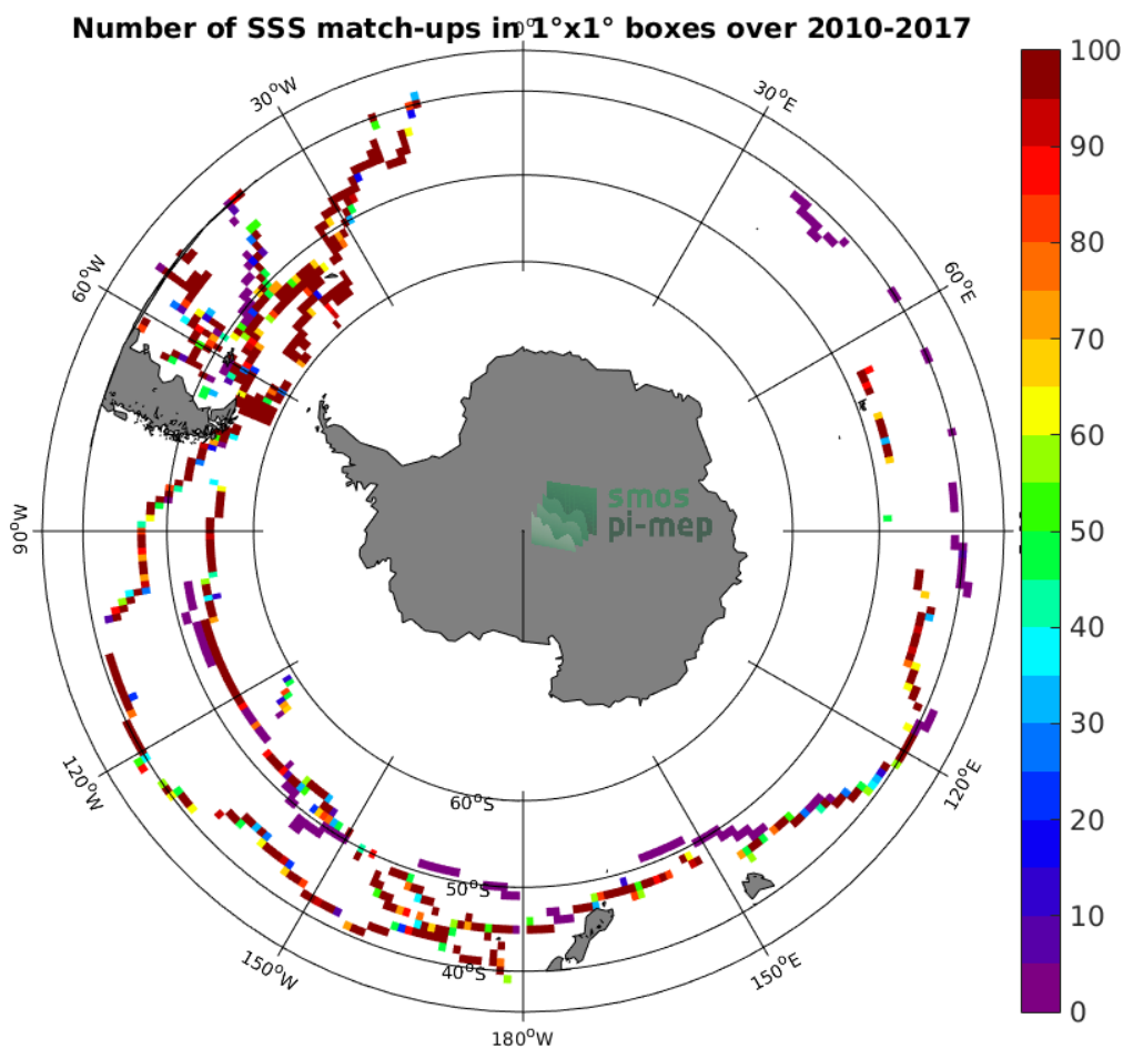
Figure 4: Number of SSS match-ups between TSG-GOSUD-Sailing-ship SSS and the SMOS L3 v2 - Daily - 0.5 Deg (CATDS-CECOS-IFREMER) SSS product for the Roaring Forties and Furious Fifties Pi-MEP region over 1°x1° boxes and for the full satellite product period.
