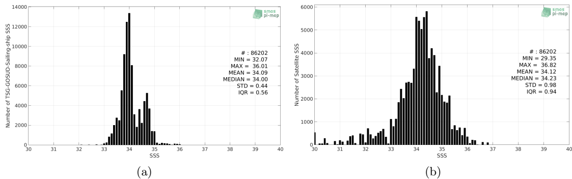
Figure 2: Histograms of SSS from TSG-GOSUD-Sailing-ship (a) and SMOS L3 v2 - Daily - 0.5 Deg (CATDS-CECOS-IFREMER) (b) considering all match-up pairs per bins of 0.1 over the Roaring Forties and Furious Fifties Pi-MEP region and for the full satellite product period.
