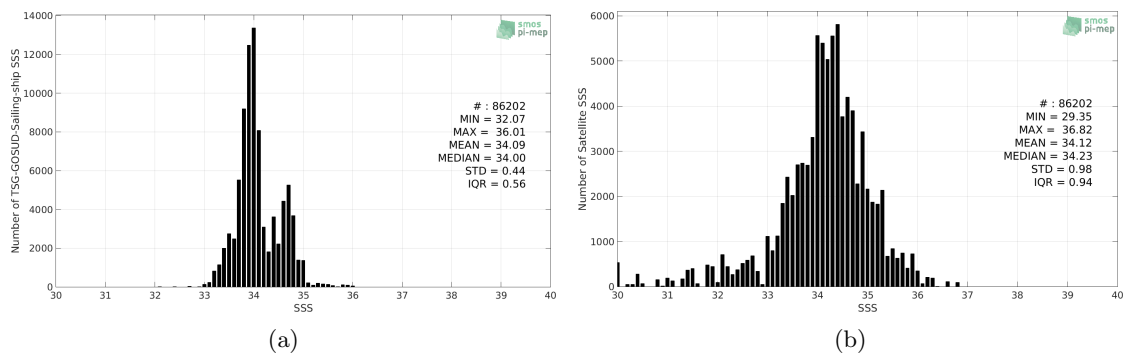
Figure 2: Histograms of SSS from TSG-GOSUD-Sailing-ship (a) and SMOS-L3-CATDS-CECOS-IFREMER-V2-1DAY-0.5DEG (b) considering all match-up pairs per bins of 0.1 over the Roaring Forties and Furious Fifties Pi-MEP region and for the full satellite product period.
