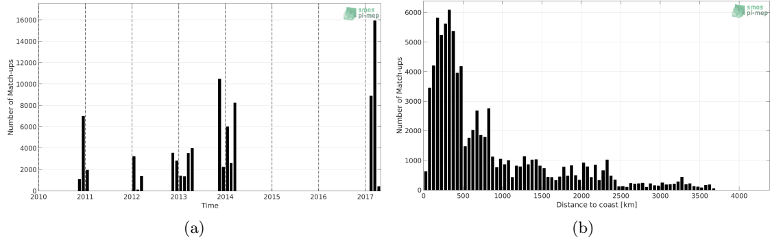
Figure 1: Number of match-ups between TSG-GOSUD-Sailing-ship and SMOS-L3-CATDS-CECOS-IFREMER-V2-1DAY-0.5DEG SSS as a function of time (a) and as function of the distance to coast (b) over the Roaring Forties and Furious Fifties Pi-MEP region and for the full satellite product period.
