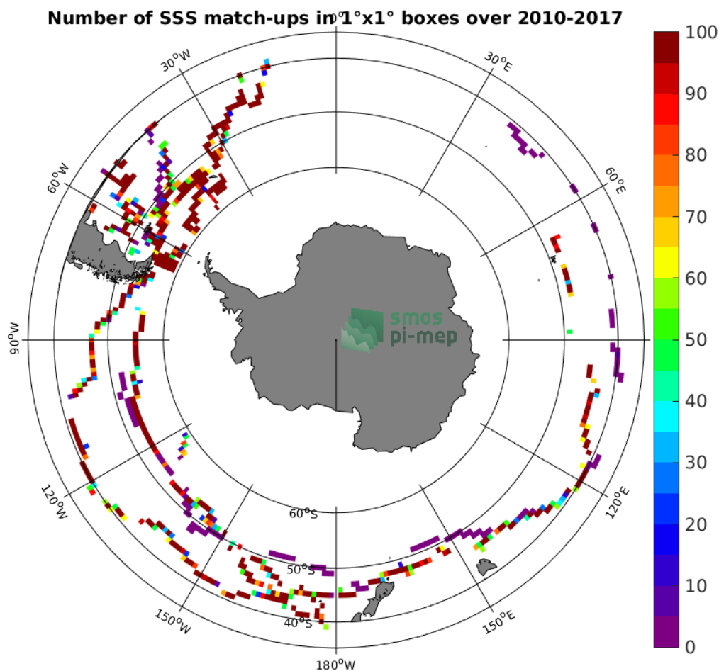
Figure 4: Number of SSS match-ups between TSG-GOSUD-Sailing-ship SSS and the SMOS-L3-CATDS-CECOS-IFREMER-V2-1DAY-0.5DEG SSS product for the Roaring Forties and Furious Fifties Pi-MEP region over 1°x1° boxes and for the full satellite product period.
