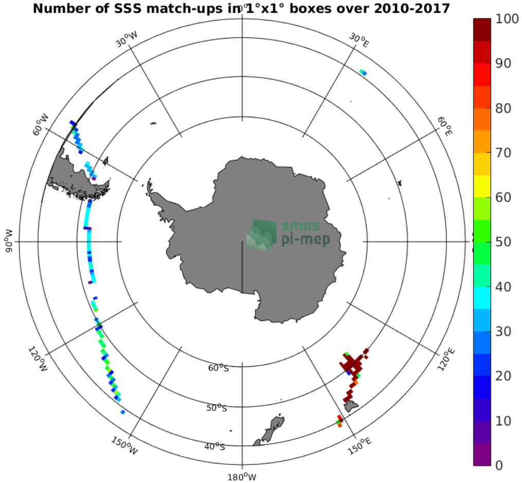
Figure 4: Number of SSS match-ups between TSG (GOSUD-Research-vessel) SSS and the SMOS SSS L3 v2 - Daily - 0.5 Deg (CATDS-CECOS-IFREMER) SSS product for the Roaring Forties and Furious Fifties Pi-MEP region over 1°x1° boxes and for the full satellite product period.
