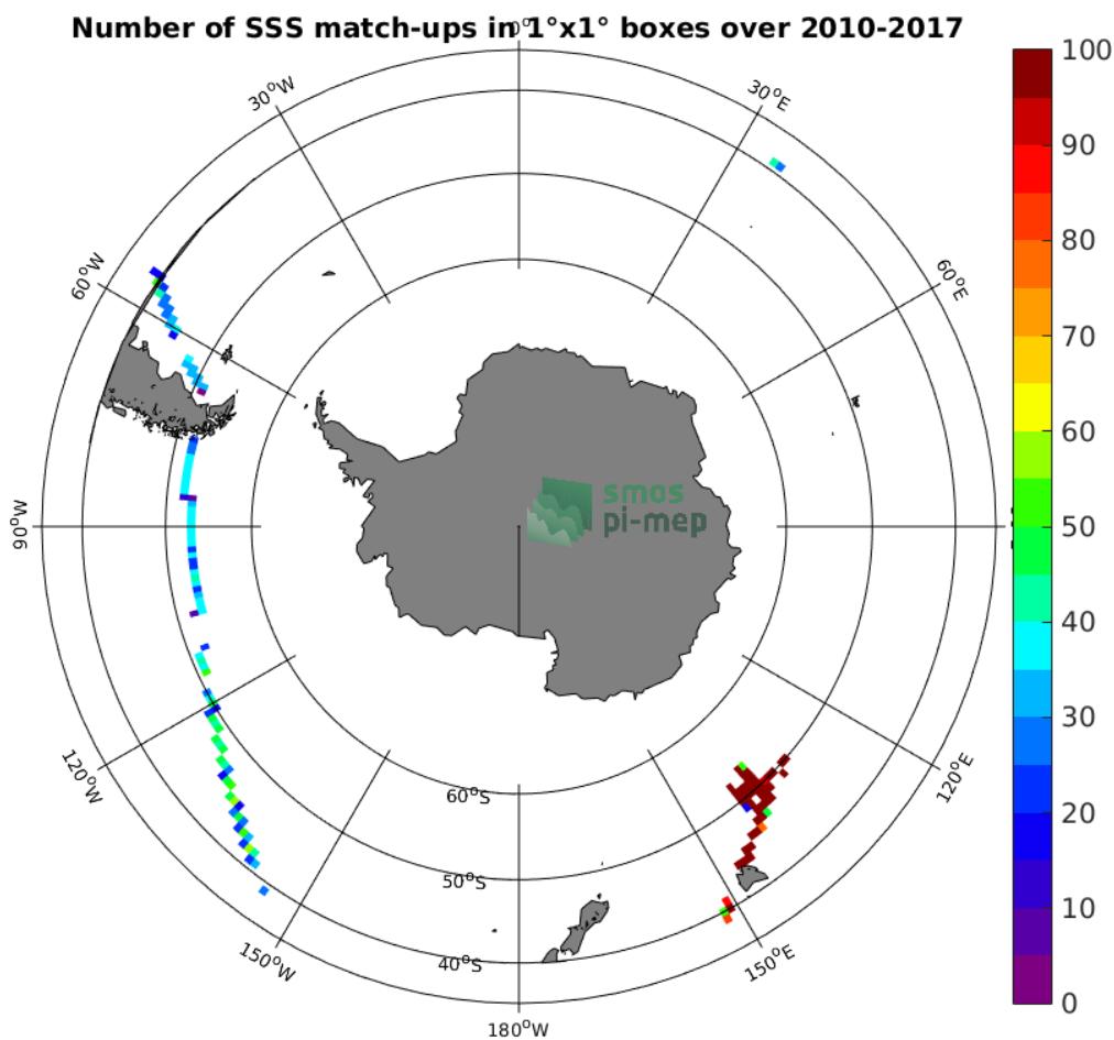
Figure 4: Number of SSS match-ups between TSG-GOSUD-Research-vessel SSS and the SMOS L3 v2 - Daily - 0.5 Deg (CATDS-CECOS-IFREMER) SSS product for the Roaring Forties and Furious Fifties Pi-MEP region over 1°x1° boxes and for the full satellite product period.
