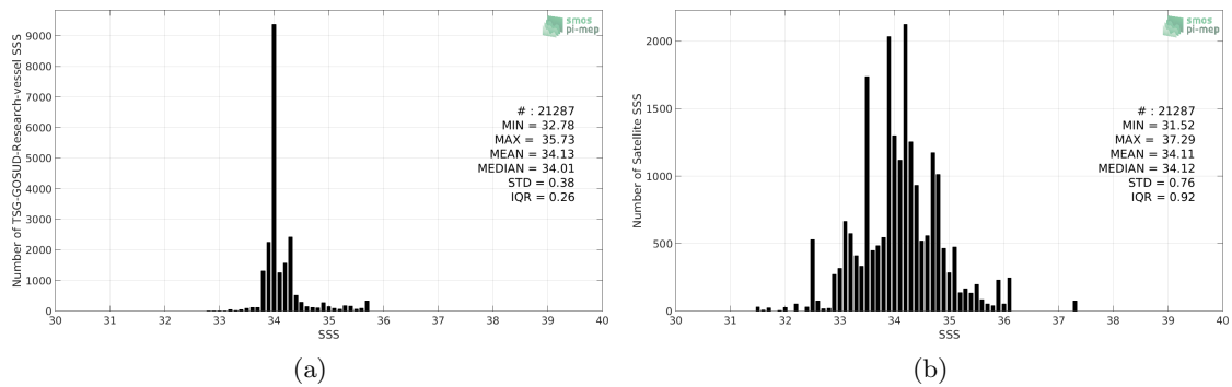
Figure 2: Histograms of SSS from TSG-GOSUD-Research-vessel (a) and SMOS L3 v2 - Daily - 0.5 Deg (CATDS-CECOS-IFREMER) (b) considering all match-up pairs per bins of 0.1 over the Roaring Forties and Furious Fifties Pi-MEP region and for the full satellite product period.
