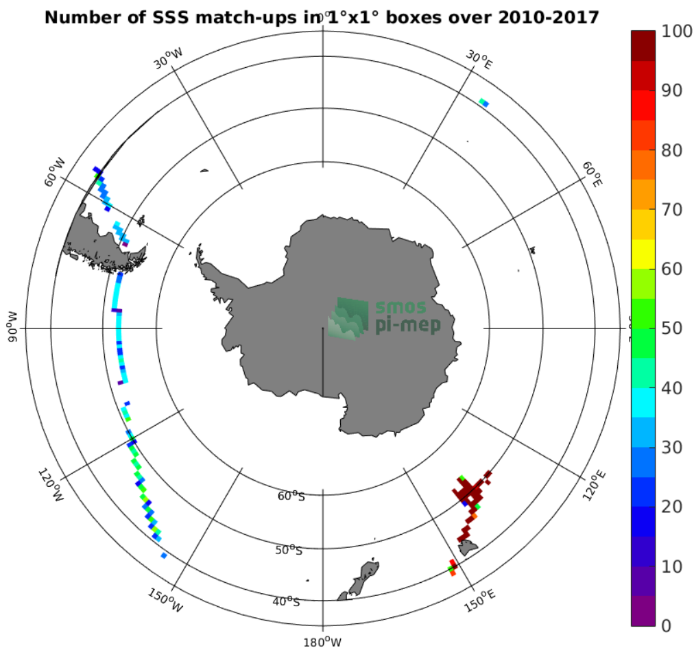
Figure 4: Number of SSS match-ups between TSG-GOSUD-Research-vessel SSS and the SMOS-L3-CATDS-CECOS-IFREMER-V2-1DAY-0.5DEG SSS product for the Roaring Forties and Furious Fifties Pi-MEP region over 1°x1° boxes and for the full satellite product period.
