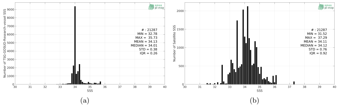
Figure 2: Histograms of SSS from TSG-GOSUD-Research-vessel (a) and SMOS-L3-CATDS-CECOS-IFREMER-V2-1DAY-0.5DEG (b) considering all match-up pairs per bins of 0.1 over the Roaring Forties and Furious Fifties Pi-MEP region and for the full satellite product period.
