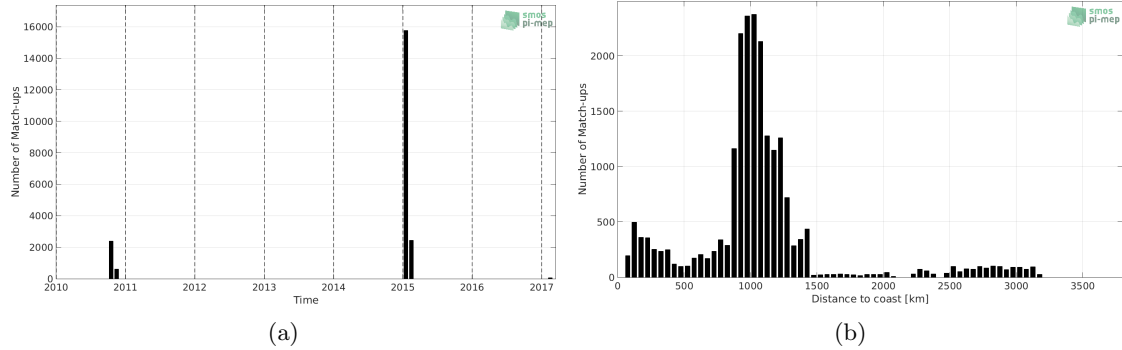
Figure 1: Number of match-ups between TSG-GOSUD-Research-vessel and SMOS-L3-CATDS-CECOS-IFREMER-V2-1DAY-0.5DEG SSS as a function of time (a) and as function of the distance to coast (b) over the Roaring Forties and Furious Fifties Pi-MEP region and for the full satellite product period.
