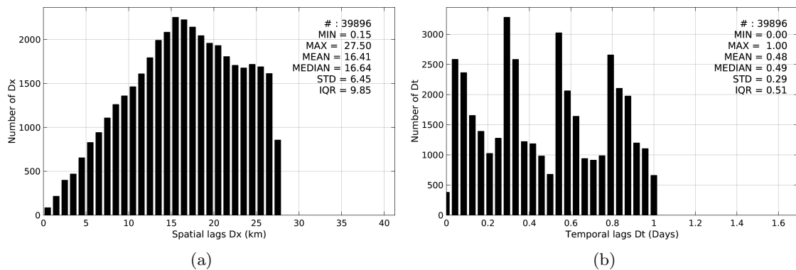
Figure 5: Histograms of the spatial (a) and temporal (b) lags between the time of the Sea mammals measurements and the date of the corresponding SMOS-L3-CATDS-CECOS-IFREMER-V2-1DAY-0.5deg SSS product.
