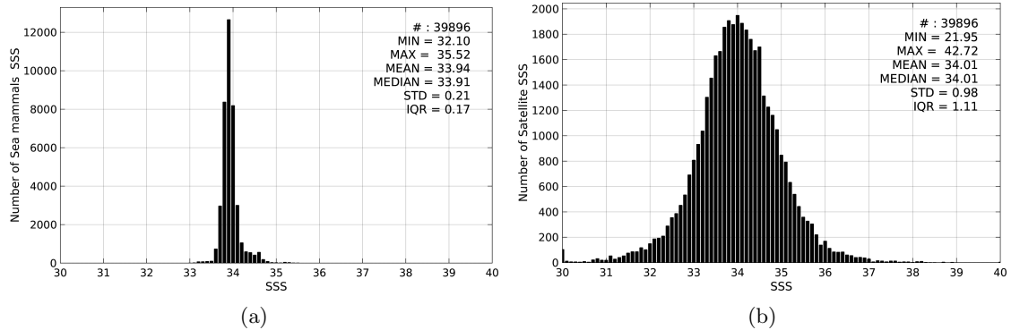
Figure 2: Histograms of SSS from Sea mammals (a) and SMOS-L3-CATDS-CECOS-IFREMER-V2-1DAY-0.5deg (b) considering all match-up pairs per bins of 0.1 over the Roaring Forties and Furious Fifties Pi-MEP region and for the full satellite product period.
