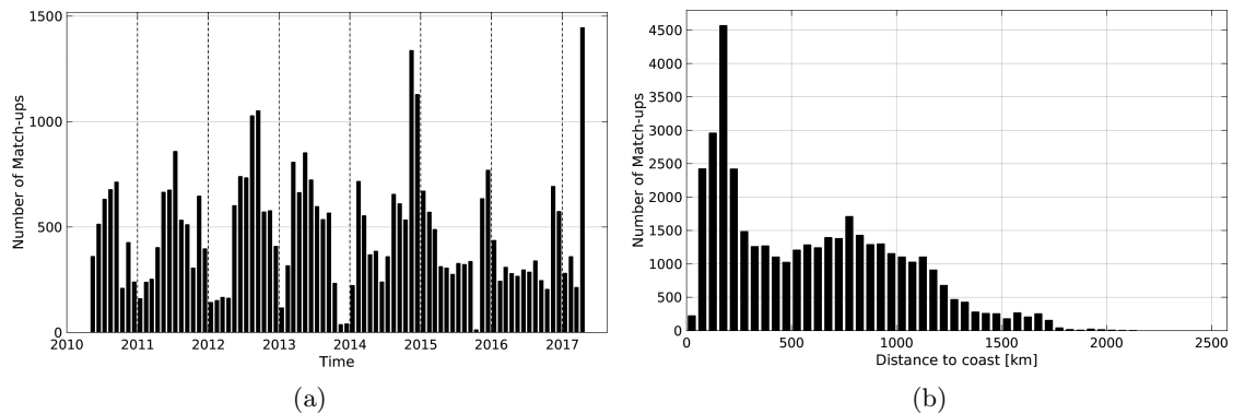
Figure 1: Number of match-ups between Sea mammals and SMOS-L3-CATDS-CECOS-IFREMER-V2-1DAY-0.5deg SSS as a function of time (a) and as function of the distance to coast (b) over the Roaring Forties and Furious Fifties Pi-MEP region and for the full satellite product period.
