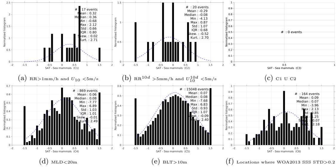
Figure 13: Normalized histogram of \Delta SSS (SMOS-L3-CATDS-CECOS-IFREMER-V2-1DAY-0.5deg - Sea mammals) for 6 different subdatasets corresponding to: RR>1mm/h and U_{10} < 5\text{m/s} (a), RR 10d >5mm/h and U_{10}^{10d} < 5\text{m/s} (b), C1 U C2 (c),MLD<20m (d),BLT>10m (e),Locations where WOA2013 SSS STD>0.2 (f).
