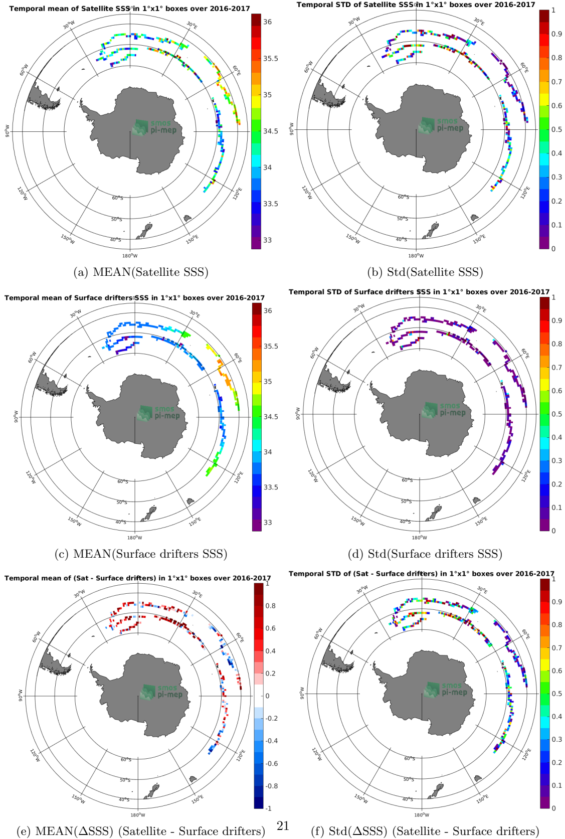
Figure 5: Temporal mean (left) and Std (right) of SSS from SMOS-L3-CATDS-CECOS-IFREMER-V2-1DAY-0.5DEG (top), Surface drifters (middle), and of \Delta SSS (Satellite - Surface drifters). Only match-up pairs are used to generate these maps.
