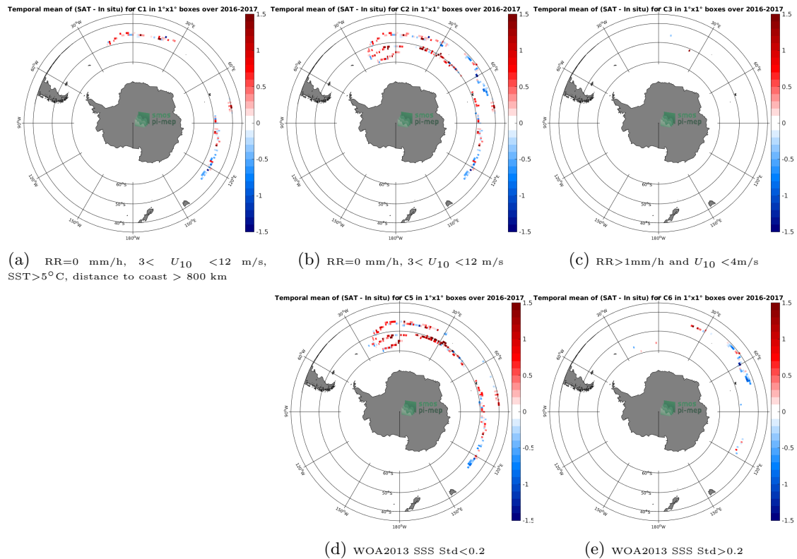
Figure 11: Temporal mean gridded over spatial boxes of size 1^\circ \times 1^\circ of \Delta SSS (SMOS-L3-CATDS-CECOS-IFREMER-V2-1DAY-0.5DEG - Surface drifters) for 5 different subdatasets corresponding to: RR=0 mm/h, 3 < U_{10} < 12 m/s, SST > 5^\circ\text{C} , distance to coast > 800 km (a), RR=0 mm/h, 3 < U_{10} < 12 m/s (b), RR > 1 mm/h and U_{10} < 4 m/s (c), WOA2013 SSS Std < 0.2 (d), WOA2013 SSS Std > 0.2 (e).
