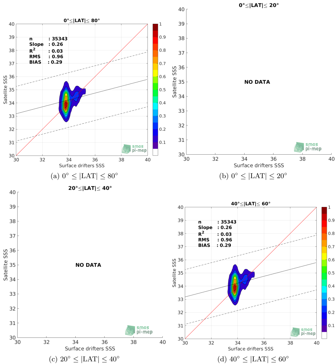
Figure 8: Contour maps of the concentration of SMOS-L3-CATDS-CECOS-IFREMER-V2-1DAY-0.5DEG SSS (y-axis) versus Surface drifters SSS (x-axis) at match-up pairs for different latitude bands. For each plot, the red line shows x=y . The black thin and dashed lines indicate a linear fit through the data cloud and the \pm 95\% confidence levels, respectively. The number match-up pairs n , the slope and R^2 coefficient of the linear fit, the root mean square (RMS) and the mean bias between satellite and in situ data are indicated for each latitude band in each plots.
