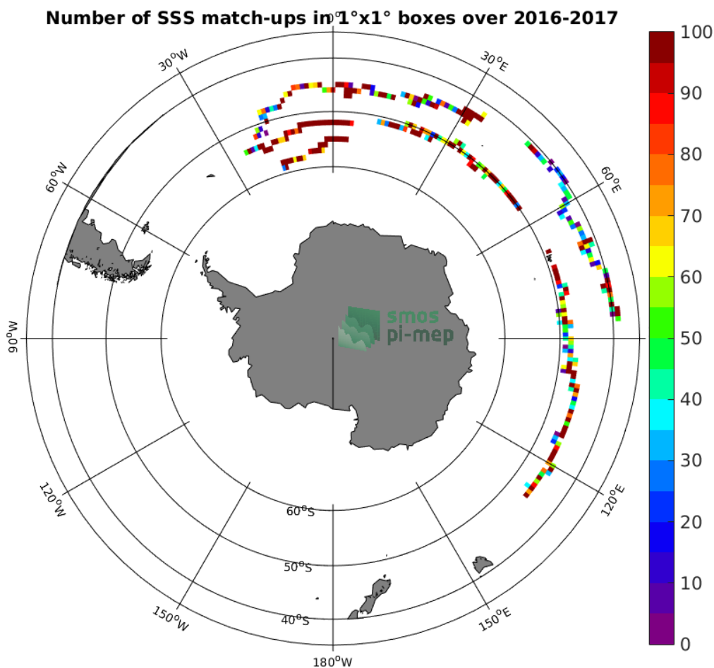
Figure 3: Number of SSS match-ups between Surface drifters SSS and the SMOS-L3-CATDS-CECOS-IFREMER-V2-1DAY-0.5DEG SSS product for the Roaring Forties and Furious Fifties Pi-MEP region over 1°x1° boxes and for the full satellite product period.
