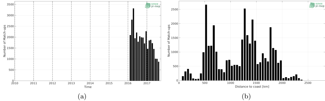
Figure 1: Number of match-ups between Surface drifters and SMOS-L3-CATDS-CECOS-IFREMER-V2-1DAY-0.5DEG SSS as a function of time (a) and as function of the distance to coast (b) over the Roaring Forties and Furious Fifties Pi-MEP region and for the full satellite product period.
