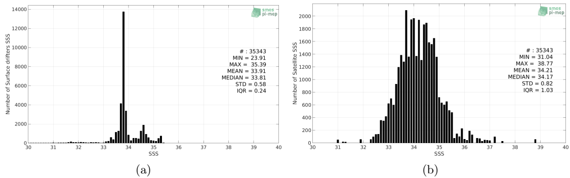
Figure 2: Histograms of SSS from Surface drifters (a) and SMOS-L3-CATDS-CECOS-IFREMER-V2-1DAY-0.5DEG (b) considering all match-up pairs per bins of 0.1 over the Roaring Forties and Furious Fifties Pi-MEP region and for the full satellite product period.
