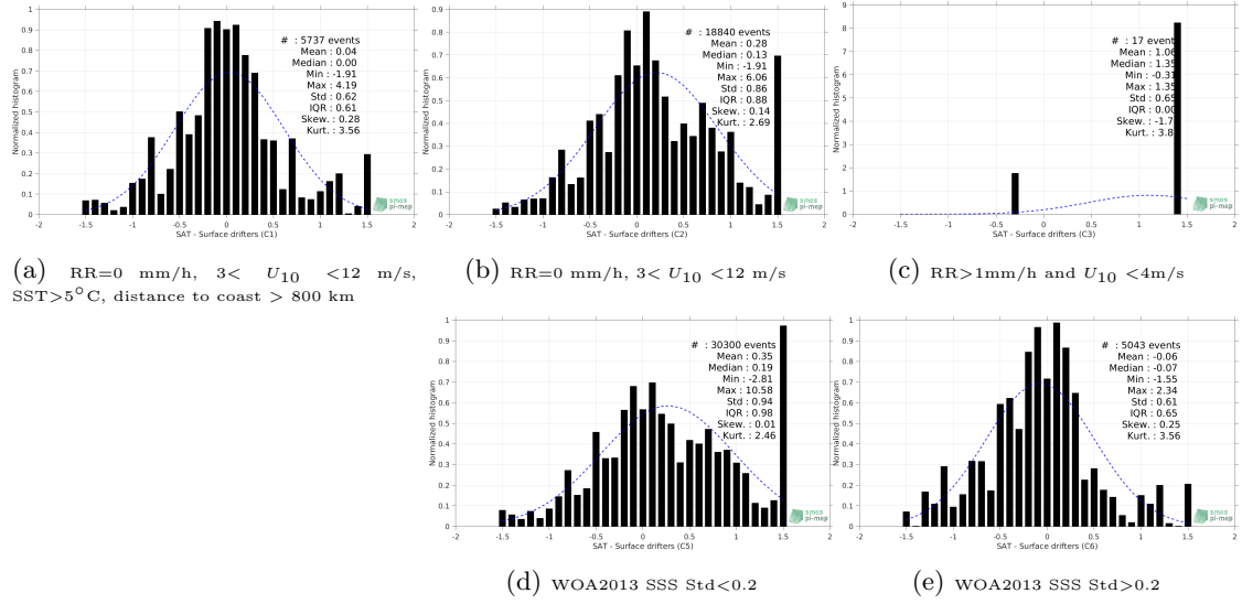
Figure 12: Normalized histogram of \Delta SSS (SMOS-L3-CATDS-CECOS-IFREMER-V2-1DAY-0.5DEG - Surface drifters) for 5 different subdatasets corresponding to: RR=0 mm/h, 3 < U_{10} < 12 m/s, SST>5°C, distance to coast > 800 km (a), RR=0 mm/h, 3 < U_{10} < 12 m/s (b), RR>1mm/h and U_{10} < 4 m/s (c), WOA2013 SSS Std<0.2 (d), WOA2013 SSS Std>0.2 (e).
