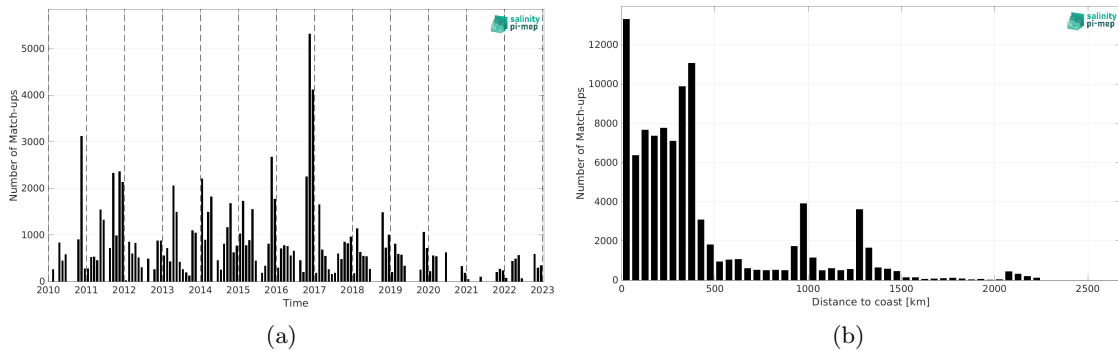
Figure 1: Number of match-ups between TSG (SAMOS) and SMOS SSS L3 v335 - Monthly - 25 km (CATDS-CPDC) SSS as a function of time (a) and as function of the distance to coast (b) over the Roaring Forties and Furious Fifties Pi-MEP region and for the full satellite product period.
