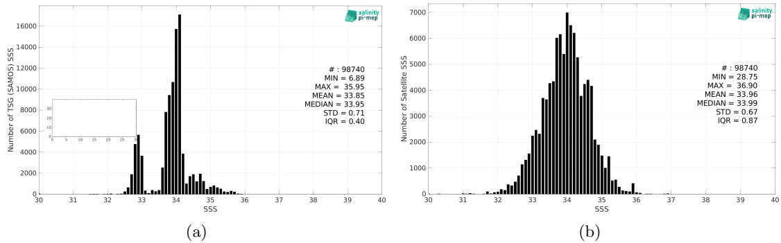
Figure 2: Histograms of SSS from TSG (SAMOS) (a) and SMOS SSS L3 v335 - Monthly - 25 km (CATDS-CPDC) (b) considering all match-up pairs per bins of 0.1 over the Roaring Forties and Furious Fifties Pi-MEP region and for the full satellite product period.
