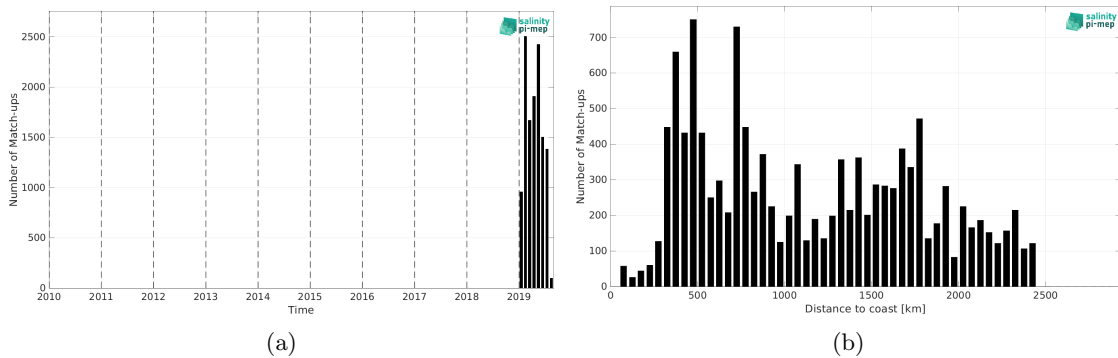
Figure 1: Number of match-ups between Saildrone and SMOS SSS L3 v335 - Monthly - 25 km (CATDS-CPDC) SSS as a function of time (a) and as function of the distance to coast (b) over the Roaring Forties and Furious Fifties Pi-MEP region and for the full satellite product period.
