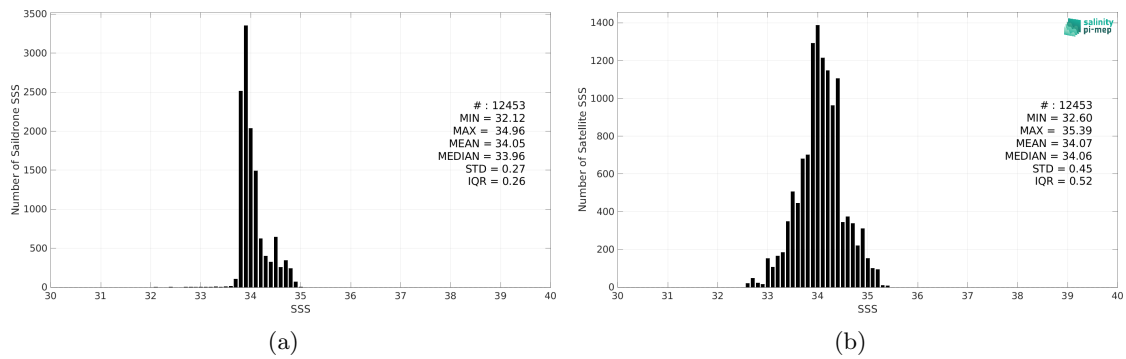
Figure 2: Histograms of SSS from Saildrone (a) and SMOS SSS L3 v335 - Monthly - 25 km (CATDS-CPDC) (b) considering all match-up pairs per bins of 0.1 over the Roaring Forties and Furious Fifties Pi-MEP region and for the full satellite product period.
