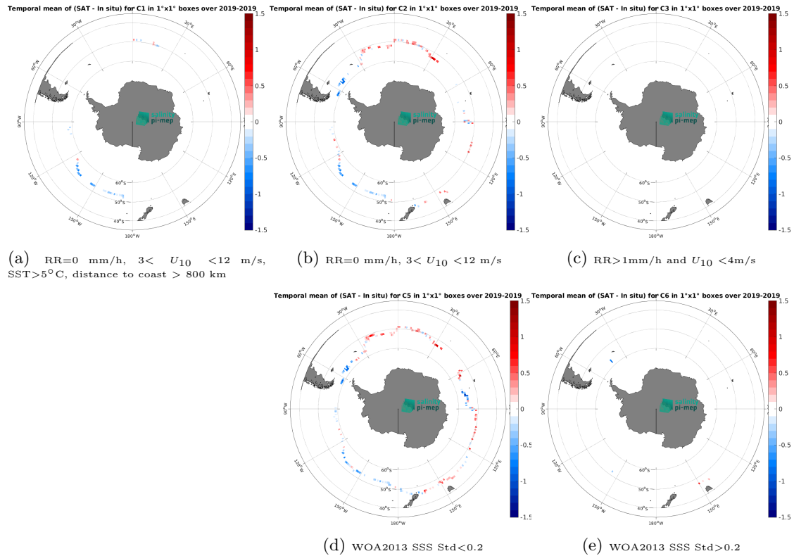
Figure 12: Temporal mean gridded over spatial boxes of size 1^{\circ}\times 1^{\circ} of \Delta\text{SSS} (SMOS SSS L3 v335 - Monthly - 25 km (CATDS-CPDC) - Saildrone) for 5 different subdatasets corresponding to:RR=0 mm/h, 3 < U_{10} < 12 m/s, SST >5^{\circ}\text{C} , distance to coast > 800 km (a), RR=0 mm/h, 3 < U_{10} < 12 m/s (b), RR >1 mm/h and U_{10} < 4 m/s (c), WOA2013 SSS Std <0.2 (d), WOA2013 SSS Std >0.2 (e).
