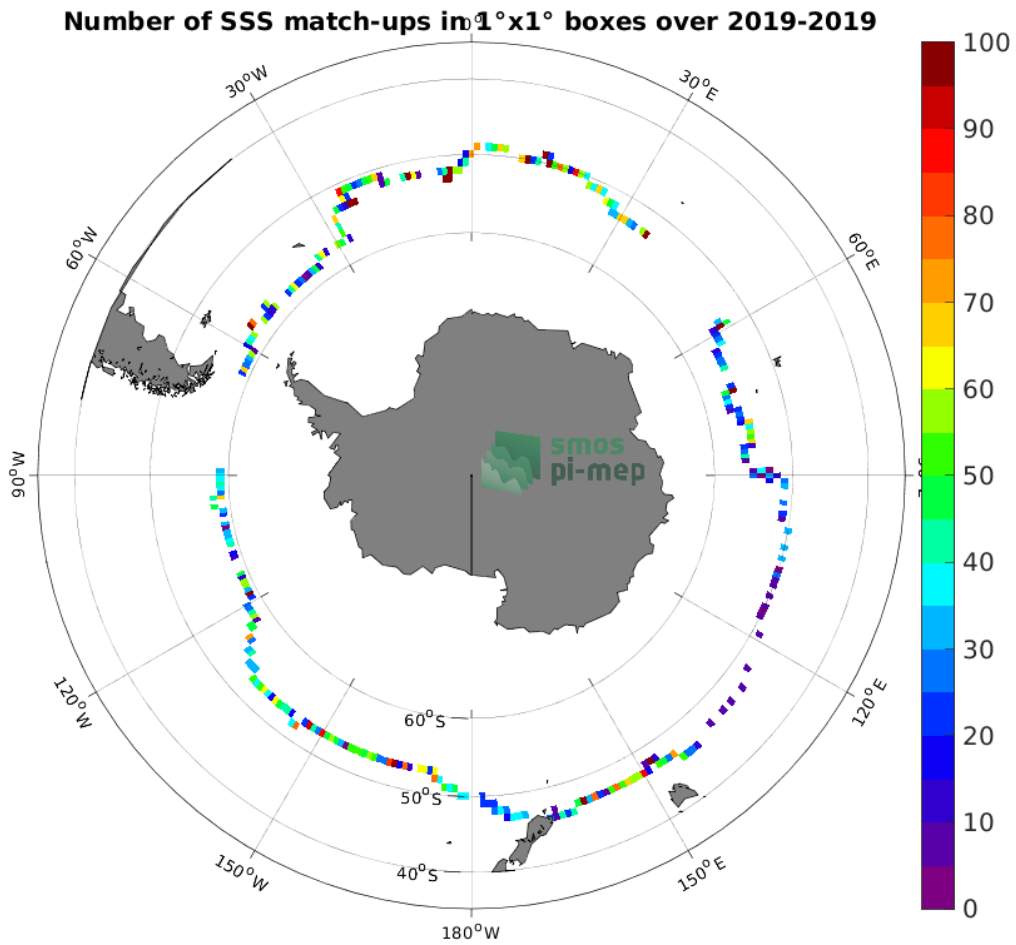
Figure 4: Number of SSS match-ups between Saildrone SSS and the SMOS SSS L3 v335 - Monthly - 25 km (CATDS-CPDC) SSS product for the Roaring Forties and Furious Fifties Pi-MEP region over 1^\circ \times 1^\circ boxes and for the full satellite product period.
