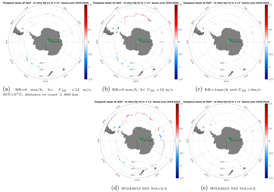
Figure 12: Temporal mean gridded over spatial boxes of size 1^{\circ}\times 1^{\circ} of \Delta\text{SSS} (SMOS SSS L3 v335 - Monthly - 25 km (CATDS-CPDC) - Saldron) for 5 different subdatasets corresponding to:RR=0 mm/h, 3 < U_{10} < 12 m/s, SST >5^{\circ}\text{C} , distance to coast > 800 km (a), RR=0 mm/h, 3 < U_{10} < 12 m/s (b), RR >1 mm/h and U_{10} < 4 m/s (c), WOA2013 SSS Std <0.2 (d), WOA2013 SSS Std >0.2 (e).
