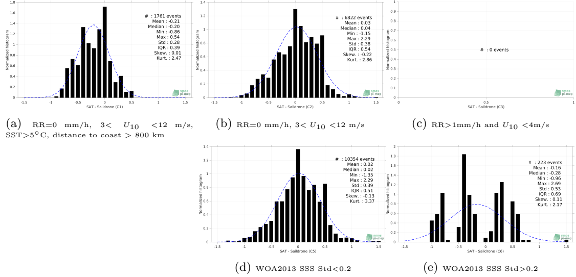
Figure 13: Normalized histogram of \Delta SSS (SMOS SSS L3 v335 - Monthly - 25 km (CATDS-CPDC) - Salldrone) for 5 different subdatasets corresponding to: RR=0 mm/h, 3 < U_{10} < 12 m/s, SST > 5°C, distance to coast > 800 km (a), RR=0 mm/h, 3 < U_{10} < 12 m/s (b), RR > 1mm/h and U_{10} < 4 m/s (c), WOA2013 SSS Std < 0.2 (d), WOA2013 SSS Std > 0.2 (e).
