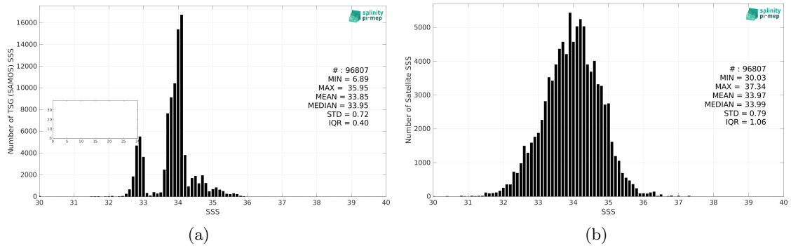
Figure 2: Histograms of SSS from TSG (SAMOS) (a) and SMOS SSS L3 v335 - 10 Days - 25 km (CATDS-CPDC) (b) considering all match-up pairs per bins of 0.1 over the Roaring Forties and Furious Fifties Pi-MEP region and for the full satellite product period.
