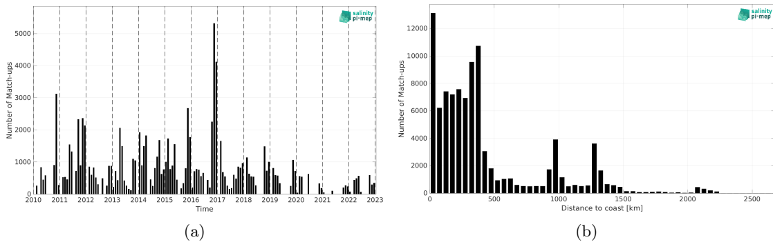
Figure 1: Number of match-ups between TSG (SAMOS) and SMOS SSS L3 v335 - 10 Days - 25 km (CATDS-CPDC) SSS as a function of time (a) and as function of the distance to coast (b) over the Roaring Forties and Furious Fifties Pi-MEP region and for the full satellite product period.
