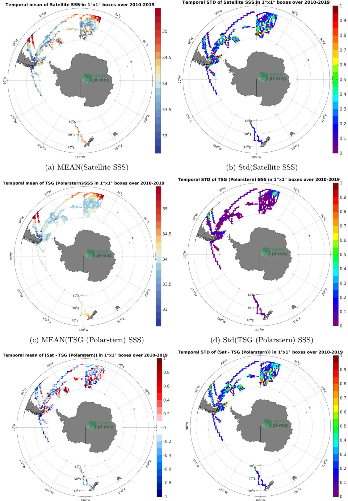
Figure 6: Temporal mean (left) and Std (right) of SSS from SMOS SSS L3 v335 - 10 Days - 25 km (CATDS-CPDC) (top), TSG (Polarstern) (middle), and of \Delta SSS (Satellite - TSG (Polarstern)). Only match-up pairs are used to generate these maps.
