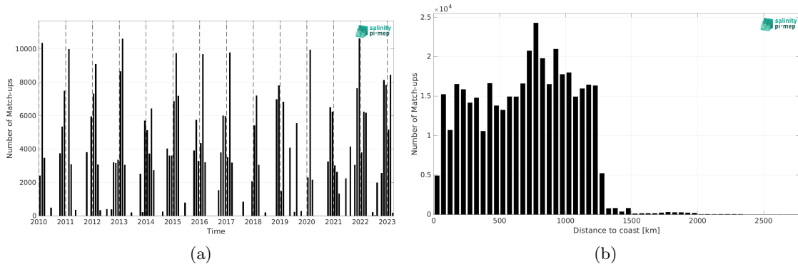
Figure 2: Number of match-ups between TSG (LEGOS-DM) and SMOS SSS L3 v335 - 10 Days - 25 km (CATDS-CPDC) SSS as a function of time (a) and as function of the distance to coast (b) over the Roaring Forties and Furious Fifties Pi-MEP region and for the full satellite product period.
