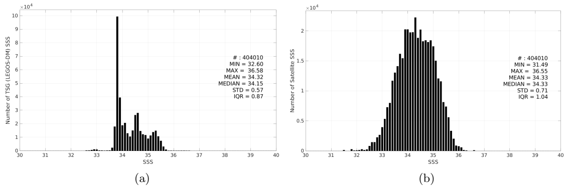
Figure 3: Histograms of SSS from TSG (LEGOS-DM) (a) and SMOS SSS L3 v335 - 10 Days - 25 km (CATDS-CPDC) (b) considering all match-up pairs per bins of 0.1 over the Roaring Forties and Furious Fifties Pi-MEP region and for the full satellite product period.
