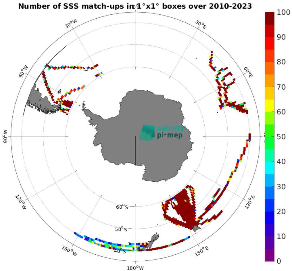
Figure 5: Number of SSS match-ups between TSG (LEGOS-DM) SSS and the SMOS SSS L3 v335 - 10 Days - 25 km (CATDS-CPDC) SSS product for the Roaring Forties and Furious Fifties Pi-MEP region over 1^\circ \times 1^\circ boxes and for the full satellite product period.
