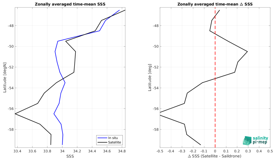
Figure 9: Left panel: Zonal mean SSS from SMOS SSS L3 v335 - 10 Days - 25 km (CATDS-CPDC) satellite product (black) and from Sailldrone (blue). Right panel: Zonal mean of \Delta SSS (Satellite - Sailldrone) for all the collected Pi-MEP match-up pairs estimated over the full satellite product period.
