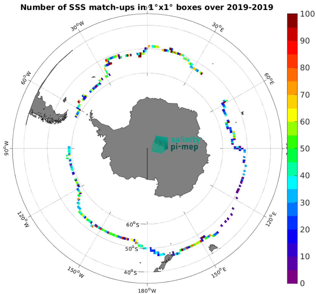
Figure 4: Number of SSS match-ups between Saildrone SSS and the SMOS SSS L3 v335 - 10 Days - 25 km (CATDS-CPDC) SSS product for the Roaring Forties and Furious Fifties Pi-MEP region over 1^{\circ} \times 1^{\circ} boxes and for the full satellite product period.
