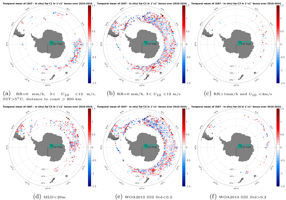
Figure 14: Temporal mean gridded over spatial boxes of size 1^\circ \times 1^\circ of \Delta\text{SSS} (SMOS SSS L3 v335 - 10 Days - 25 km (CATDS-CPDC) - Marine mammals) for 6 different subdatasets corresponding to:RR=0 mm/h, 3 < U_{10} < 12 m/s, SST>5°C, distance to coast > 800 km (a), RR=0 mm/h, 3 < U_{10} < 12 m/s (b), RR>1mm/h and U_{10} < 4 m/s (c),MLD<20m (d),WOA2013 SSS Std<0.2 (e),WOA2013 SSS Std>0.2 (f).
