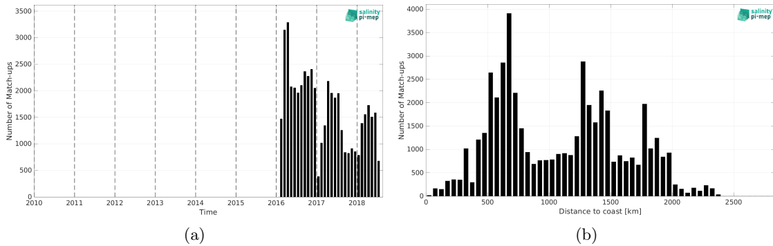
Figure 2: Number of match-ups between Surface drifters and SMOS SSS L3 v335 - 10 Days - 25 km (CATDS-CPDC) SSS as a function of time (a) and as function of the distance to coast (b) over the Roaring Forties and Furious Fifties Pi-MEP region and for the full satellite product period.
