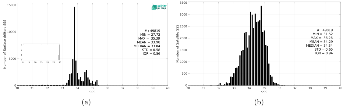
Figure 3: Histograms of SSS from Surface drifters (a) and SMOS SSS L3 v335 - 10 Days - 25 km (CATDS-CPDC) (b) considering all match-up pairs per bins of 0.1 over the Roaring Forties and Furious Fifties Pi-MEP region and for the full satellite product period.
