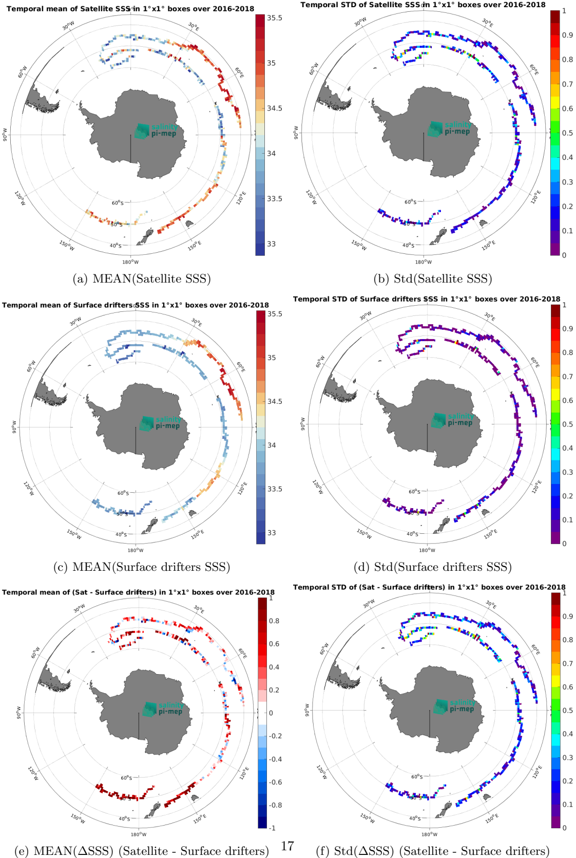
Figure 6: Temporal mean (left) and Std (right) of SSS from SMOS SSS L3 v335 - 10 Days - 25 km (CATDS-CPDC) (top), Surface drifters (middle), and of \Delta SSS (Satellite - Surface drifters). Only match-up pairs are used to generate these maps.
