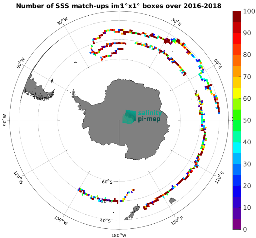
Figure 4: Number of SSS match-ups between Surface drifters SSS and the SMOS SSS L3 v335 - 10 Days - 25 km (CATDS-CPDC) SSS product for the Roaring Forties and Furious Fifties Pi-MEP region over 1^\circ \times 1^\circ boxes and for the full satellite product period.
