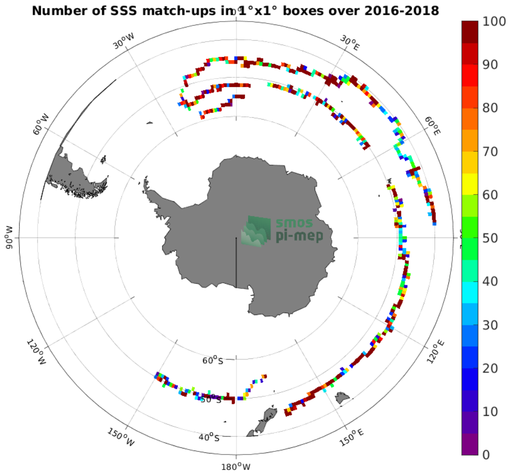
Figure 3: Number of SSS match-ups between Surface drifters SSS and the SMOS SSS L3 v335 - 10 Days - 25 km (CATDS-CPDC) SSS product for the Roaring Forties and Furious Fifties Pi-MEP region over 1^\circ \times 1^\circ boxes and for the full satellite product period.
