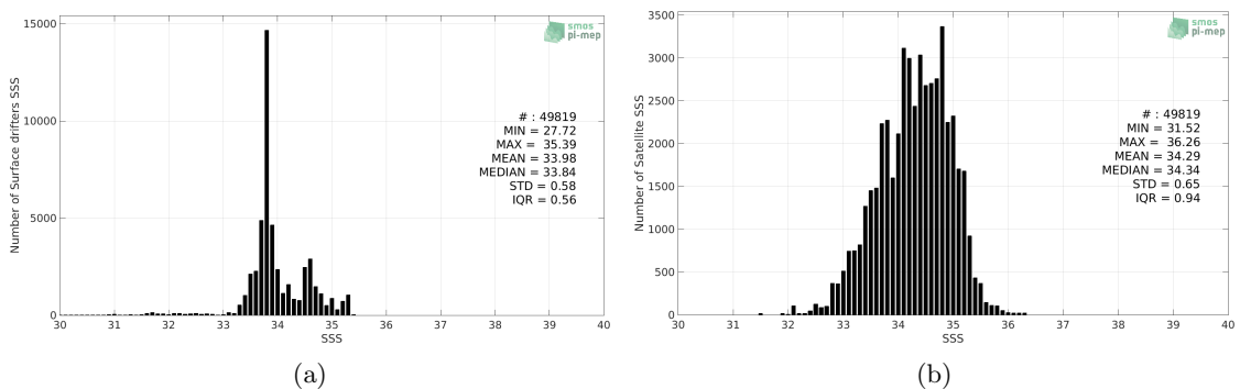
Figure 2: Histograms of SSS from Surface drifters (a) and SMOS SSS L3 v335 - 10 Days - 25 km (CATDS-CPDC) (b) considering all match-up pairs per bins of 0.1 over the Roaring Forties and Furious Fifties Pi-MEP region and for the full satellite product period.
