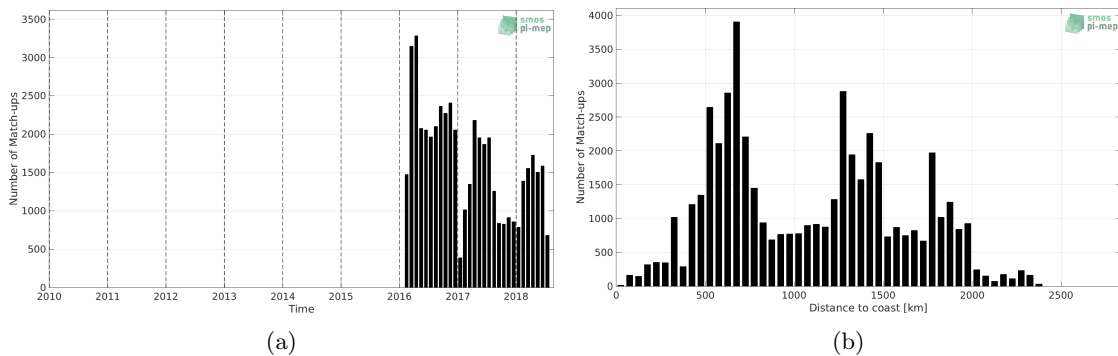
Figure 1: Number of match-ups between Surface drifters and SMOS SSS L3 v335 - 10 Days - 25 km (CATDS-CPDC) SSS as a function of time (a) and as function of the distance to coast (b) over the Roaring Forties and Furious Fifties Pi-MEP region and for the full satellite product period.
