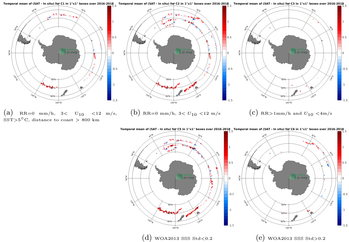
Figure 11: Temporal mean gridded over spatial boxes of size 1^{\circ}\times 1^{\circ} of \Delta\text{SSS} (SMOS SSS L3 v335 - 10 Days - 25 km (CATDS-CPDC) - Surface drifters) for 5 different subdatasets corresponding to:RR=0 mm/h, 3 < U_{10} < 12 m/s, SST >5^{\circ}\text{C} , distance to coast > 800 km (a), RR=0 mm/h, 3 < U_{10} < 12 m/s (b), RR >1 mm/h and U_{10} < 4 m/s (c), WOA2013 SSS Std <0.2 (d), WOA2013 SSS Std >0.2 (e).
