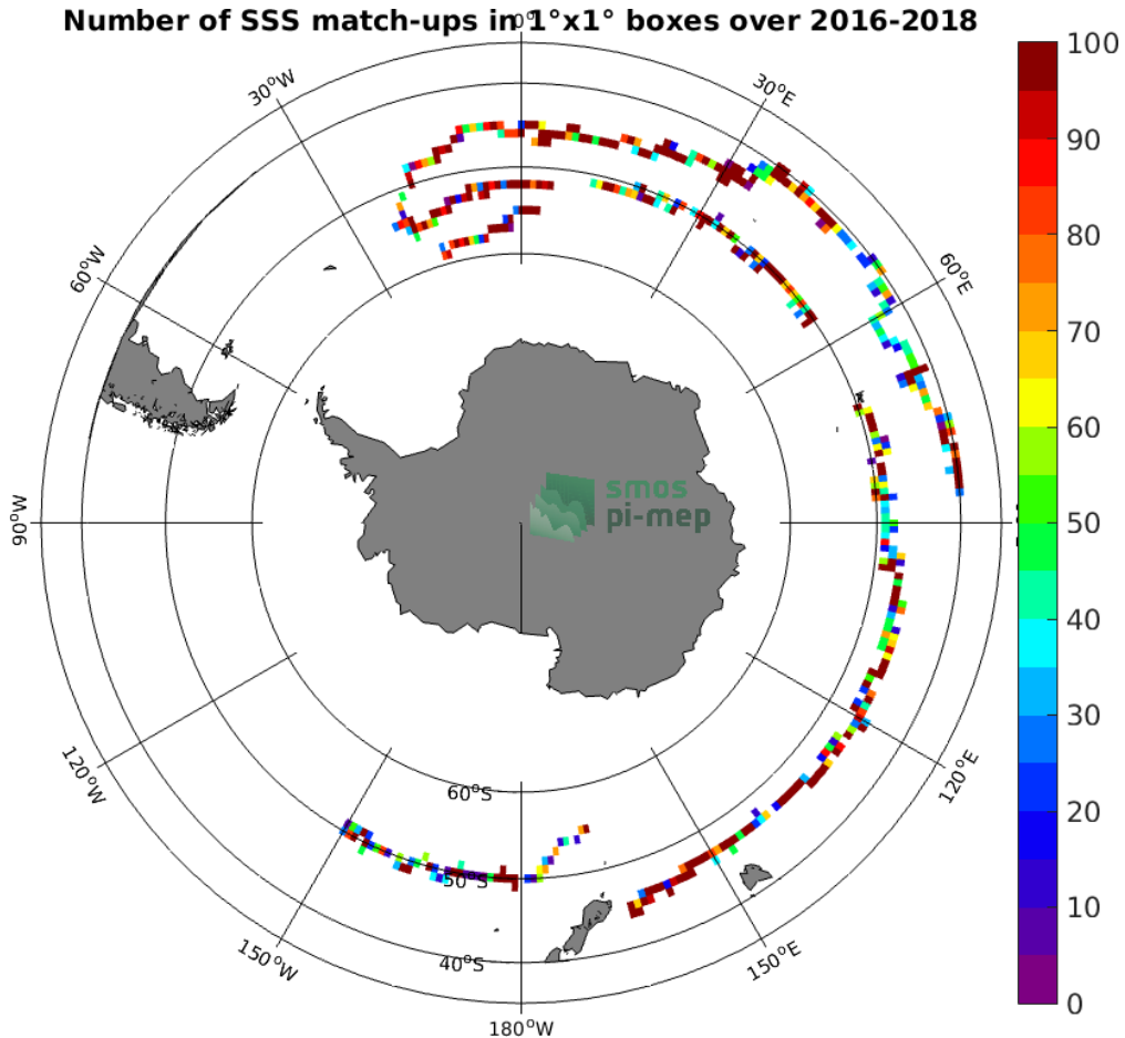
Figure 3: Number of SSS match-ups between Surface drifters SSS and the SMOS SSS L3 v335 - 10 Days - 25 km (CATDS-CPDC) SSS product for the Roaring Forties and Furious Fifties Pi-MEP region over 1^\circ \times 1^\circ boxes and for the full satellite product period.
