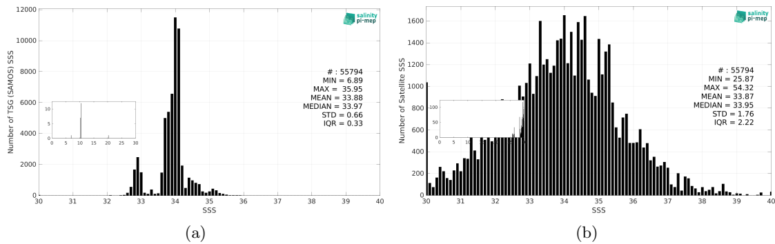
Figure 3: Histograms of SSS from TSG (SAMOS) (a) and SMOS SSS L2Q v333 - 0.25 Deg (CATDS-CPDC) (b) considering all match-up pairs per bins of 0.1 over the Roaring Forties and Furious Fifties Pi-MEP region and for the full satellite product period.
