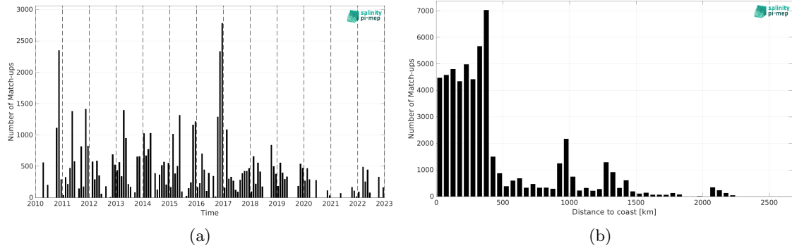
Figure 2: Number of match-ups between TSG (SAMOS) and SMOS SSS L2Q v333 - 0.25 Deg (CATDS-CPDC) SSS as a function of time (a) and as function of the distance to coast (b) over the Roaring Forties and Furious Fifties Pi-MEP region and for the full satellite product period.
