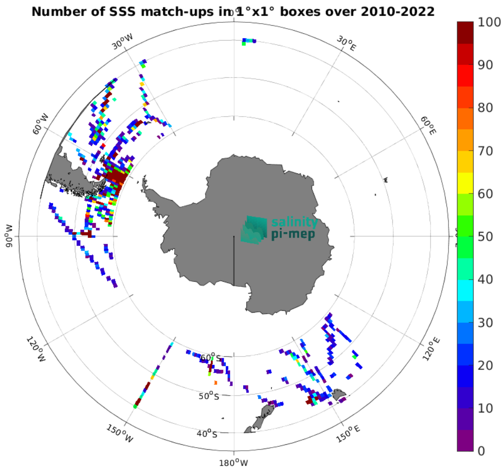
Figure 5: Number of SSS match-ups between TSG (SAMOS) SSS and the SMOS SSS L2Q v333 - 0.25 Deg (CATDS-CPDC) SSS product for the Roaring Forties and Furious Fifties Pi-MEP region over 1^{\circ} \times 1^{\circ} boxes and for the full satellite product period.
