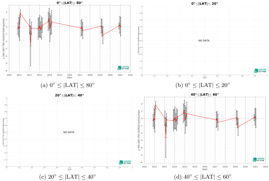
Figure 11: Monthly median (red curves) of \Delta SSS (Satellite - in situ ) between SMOS SSS L2Q v333 - 0.25 Deg (CATDS-CPDC) and TSG (GOSUD-Sailing-ship) SSS as function of time for all the collected Pi-MEP match-up pairs estimated over the Roaring Forties and Furious Fifties Pi-MEP region and for the full satellite product period are shown for different latitude bands: (a) 80^\circ\text{S}-80^\circ\text{N} , (b) 20^\circ\text{S}-20^\circ\text{N} , (c) 40^\circ\text{S}-20^\circ\text{S} and 20^\circ\text{N}-40^\circ\text{N} and (d) 60^\circ\text{S}-40^\circ\text{S} and 40^\circ\text{N}-60^\circ\text{N} .
