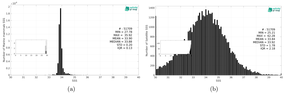
Figure 3: Histograms of SSS from Marine mammals (a) and SMOS SSS L2Q v333 - 0.25 Deg (CATDS-CPDC) (b) considering all match-up pairs per bins of 0.1 over the Roaring Forties and Furious Fifties Pi-MEP region and for the full satellite product period.
