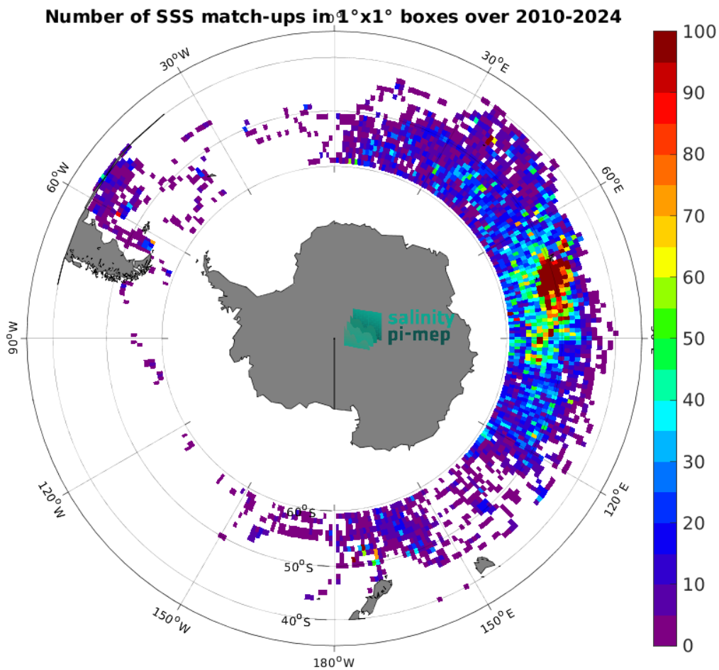
Figure 5: Number of SSS match-ups between Marine mammals SSS and the SMOS SSS L2Q v333 - 0.25 Deg (CATDS-CPDC) SSS product for the Roaring Forties and Furious Fifties Pi-MEP region over 1^\circ \times 1^\circ boxes and for the full satellite product period.
