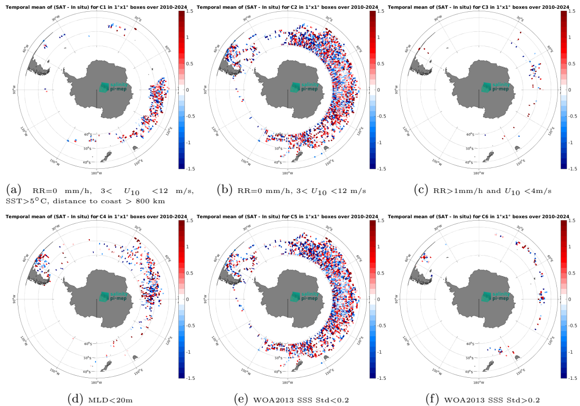
Figure 14: Temporal mean gridded over spatial boxes of size 1^\circ \times 1^\circ of \Delta\text{SSS} (SMOS SSS L2Q v333 - 0.25 Deg (CATDS-CPDC) - Marine mammals) for 6 different subdatasets corresponding to:RR=0 mm/h, 3 < U_{10} < 12 m/s, SST>5°C, distance to coast > 800 km (a), RR=0 mm/h, 3 < U_{10} < 12 m/s (b), RR>1mm/h and U_{10} < 4 m/s (c),MLD<20m (d),WOA2013 SSS Std<0.2 (e),WOA2013 SSS Std>0.2 (f).
