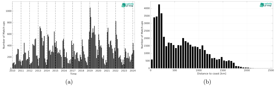
Figure 2: Number of match-ups between Marine mammals and SMOS SSS L2Q v333 - 0.25 Deg (CATDS-CPDC) SSS as a function of time (a) and as function of the distance to coast (b) over the Roaring Forties and Furious Fifties Pi-MEP region and for the full satellite product period.
