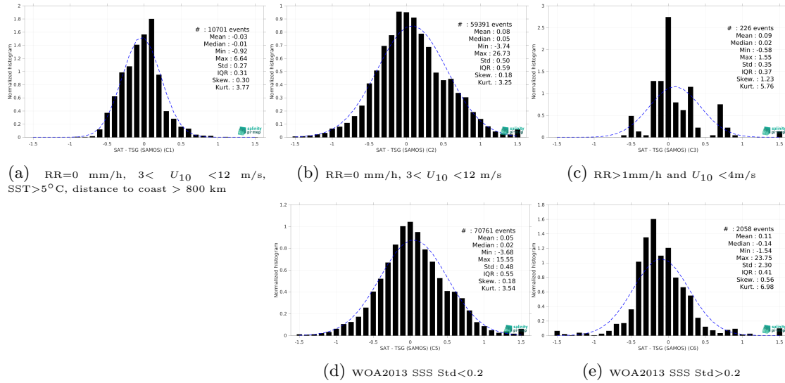
Figure 15: Normalized histogram of \Delta\text{SSS} (SMOS SSS L3 v332 - 9 Days (CATDS-CPDC) - TSG (SAMOS)) for 5 different subdatasets corresponding to: RR=0 mm/h, 3 < U_{10} < 12 m/s, SST>5°C, distance to coast > 800 km (a), RR=0 mm/h, 3 < U_{10} < 12 m/s (b), RR>1mm/h and U_{10} < 4 m/s (c), WOA2013 SSS Std<0.2 (d), WOA2013 SSS Std>0.2 (e).
