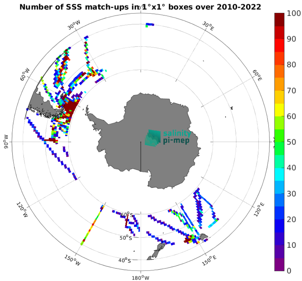
Figure 5: Number of SSS match-ups between TSG (SAMOS) SSS and the SMOS SSS L3 v332 - 9 Days (CATDS-CPDC) SSS product for the Roaring Forties and Furious Fifties Pi-MEP region over 1^{\circ} \times 1^{\circ} boxes and for the full satellite product period.
