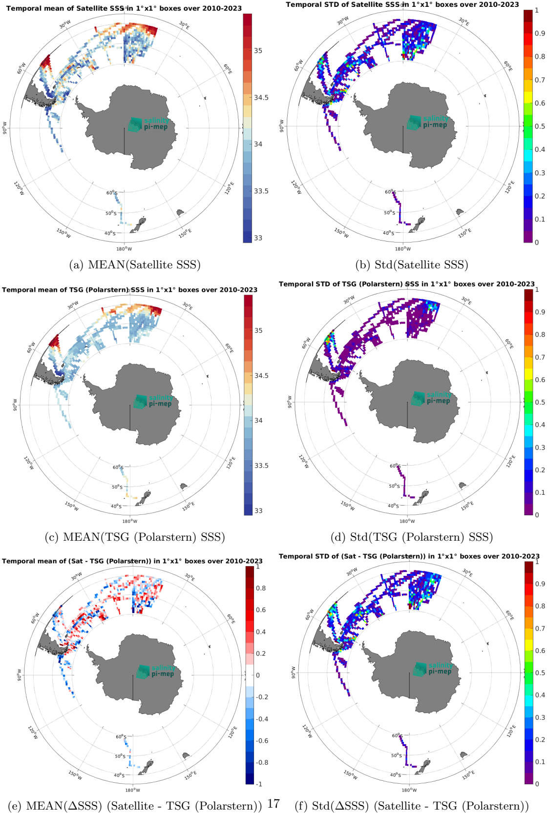
Figure 7: Temporal mean (left) and Std (right) of SSS from SMOS SSS L3 v332 - 9 Days (CATDS-CPDC) (top), TSG (Polarstern) (middle), and of \Delta SSS (Satellite - TSG (Polarstern)). Only match-up pairs are used to generate these maps.
