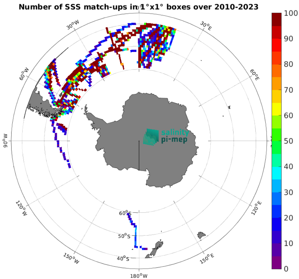
Figure 5: Number of SSS match-ups between TSG (Polarstern) SSS and the SMOS SSS L3 v332 - 9 Days (CATDS-CPDC) SSS product for the Roaring Forties and Furious Fifties Pi-MEP region over 1^\circ \times 1^\circ boxes and for the full satellite product period.
