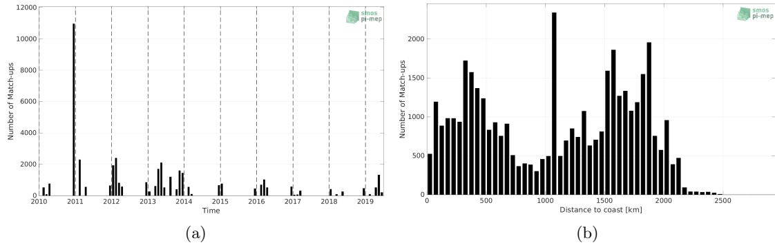
Figure 1: Number of match-ups between TSG (Polarstern) and SMOS SSS L3 v332 - 9 Days (CATDS-CPDC) SSS as a function of time (a) and as function of the distance to coast (b) over the Roaring Forties and Furious Fifties Pi-MEP region and for the full satellite product period.
