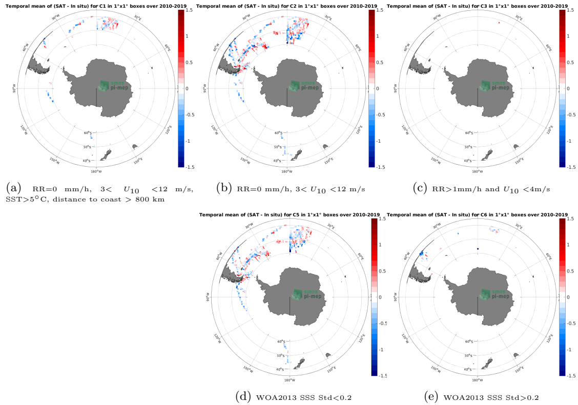
Figure 12: Temporal mean gridded over spatial boxes of size 1^{\circ} \times 1^{\circ} of \Delta\text{SSS} (SMOS SSS L3 v332 - 9 Days (CATDS-CPDC) - TSG (Polarstern)) for 5 different subdatasets corresponding to: RR=0 mm/h, 3 < U_{10} < 12 m/s, SST >5^{\circ}\text{C} , distance to coast > 800 km (a), RR=0 mm/h, 3 < U_{10} < 12 m/s (b), RR >1 mm/h and U_{10} < 4 m/s (c), WOA2013 SSS Std <0.2 (d), WOA2013 SSS Std >0.2 (e).
