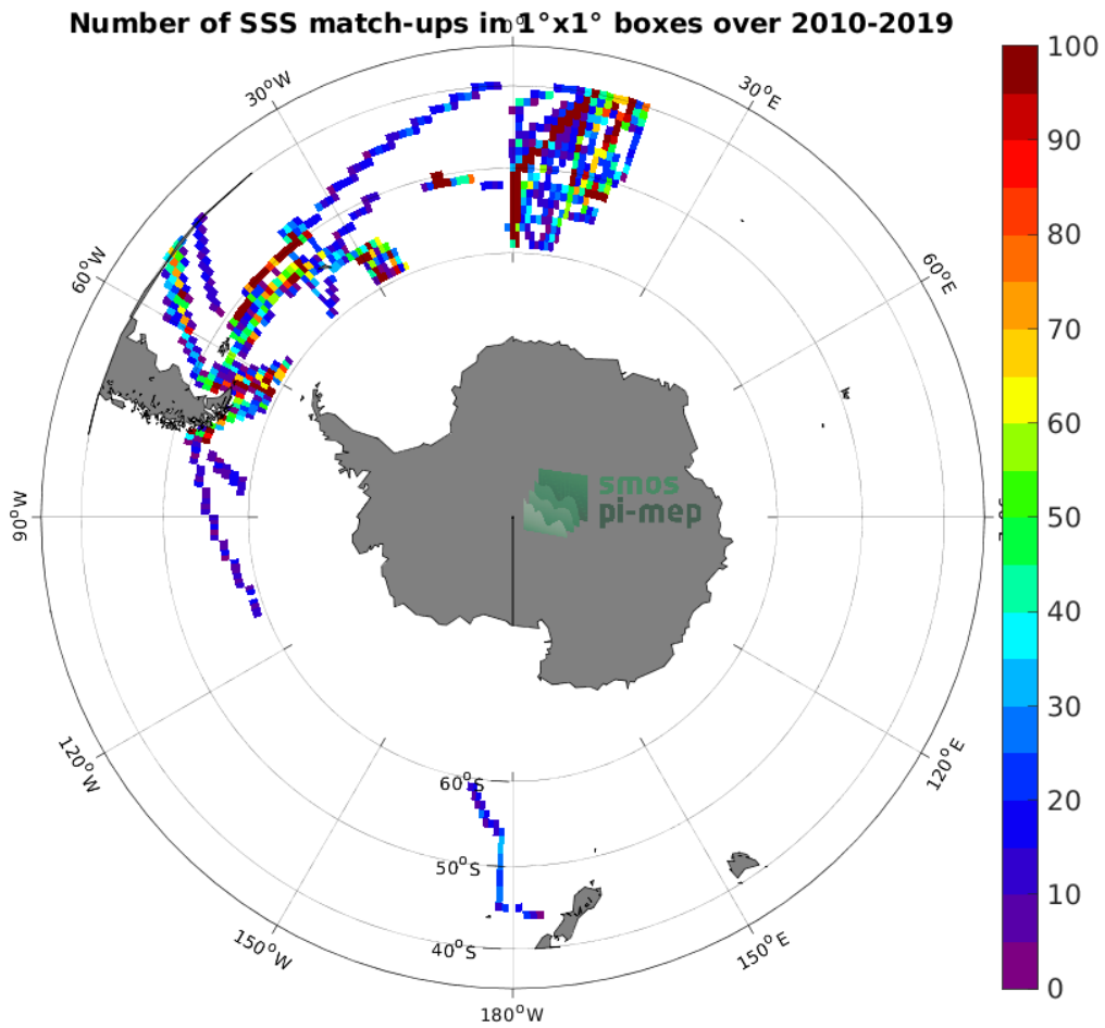
Figure 4: Number of SSS match-ups between TSG (Polarstern) SSS and the SMOS SSS L3 v332 - 9 Days (CATDS-CPDC) SSS product for the Roaring Forties and Furious Fifties Pi-MEP region over 1^\circ \times 1^\circ boxes and for the full satellite product period.
