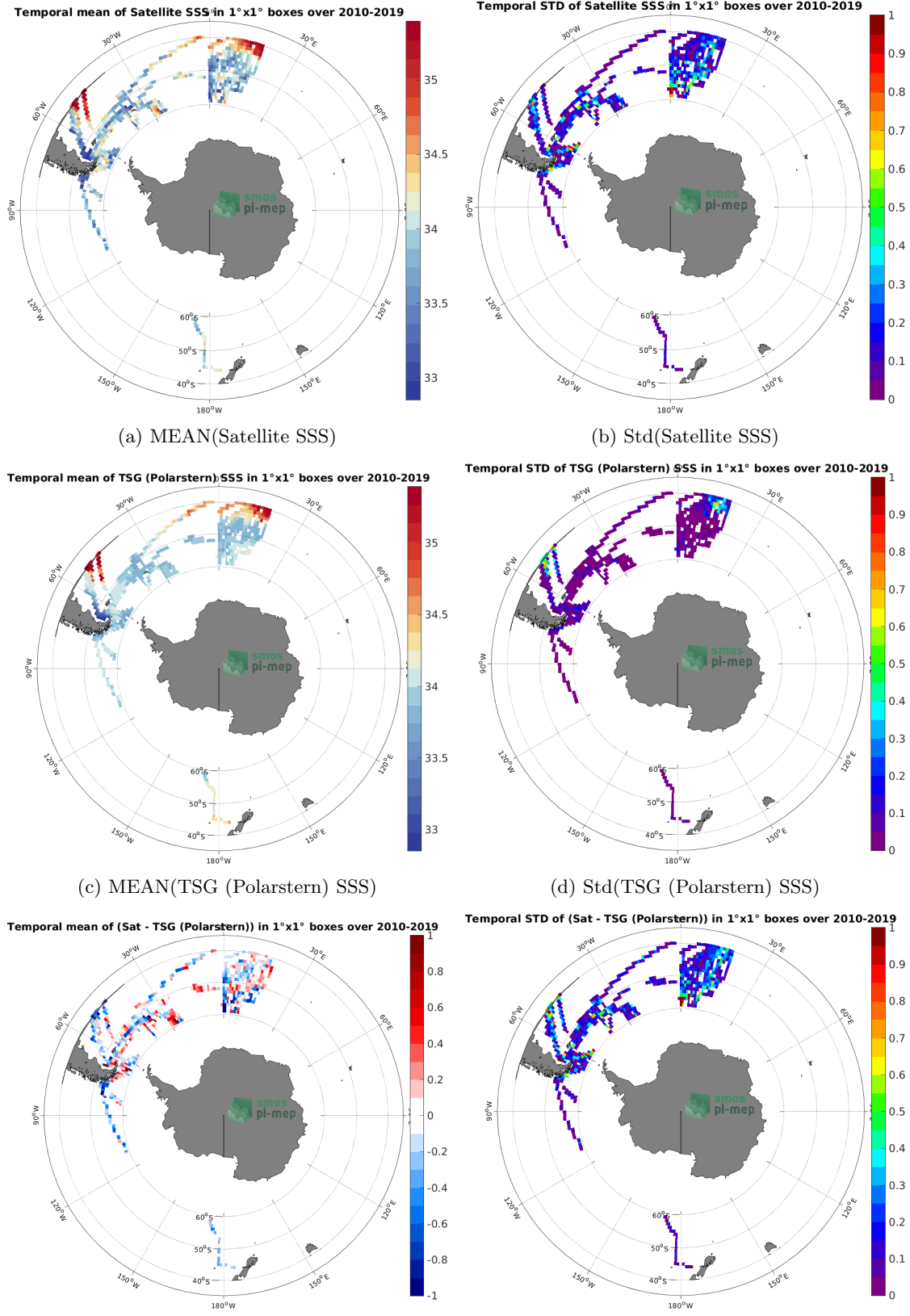
Figure 6: Temporal mean (left) and Std (right) of SSS from SMOS SSS L3 v332 - 9 Days (CATDS-CPDC) (top), TSG (Polarstern) (middle), and of \Delta SSS (Satellite - TSG (Polarstern)). Only match-up pairs are used to generate these maps.
