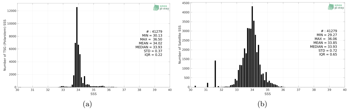
Figure 2: Histograms of SSS from TSG (Polarstern) (a) and SMOS SSS L3 v332 - 9 Days (CATDS-CPDC) (b) considering all match-up pairs per bins of 0.1 over the Roaring Forties and Furious Fifties Pi-MEP region and for the full satellite product period.
