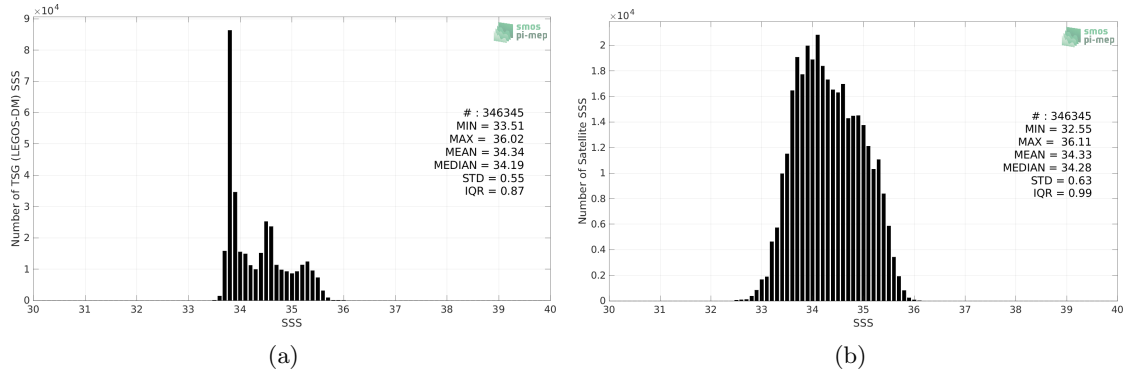
Figure 2: Histograms of SSS from TSG (LEGOS-DM) (a) and SMOS SSS L3 v332 - 9 Days (CATDS-CPDC) (b) considering all match-up pairs per bins of 0.1 over the Roaring Forties and Furious Fifties Pi-MEP region and for the full satellite product period.
