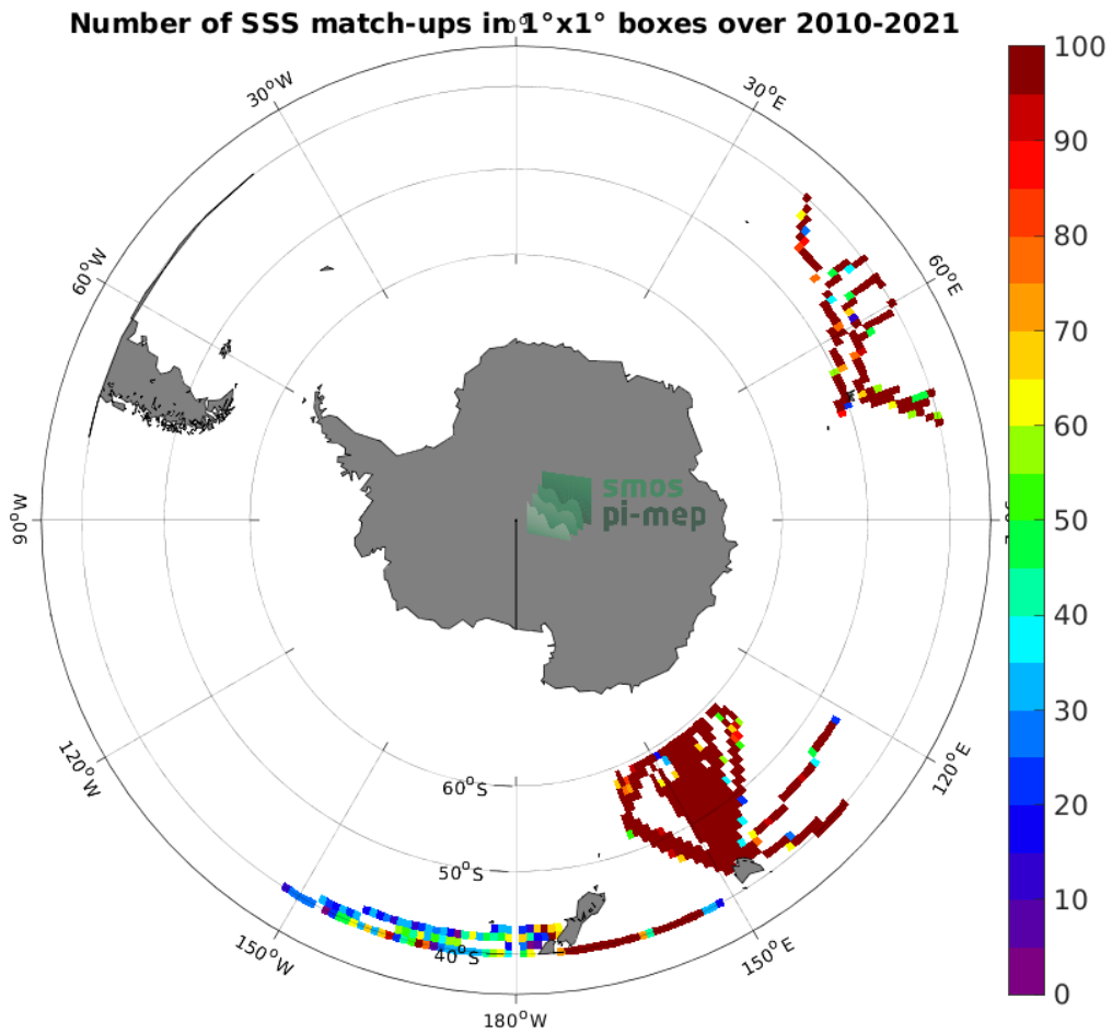
Figure 4: Number of SSS match-ups between TSG (LEGOS-DM) SSS and the SMOS SSS L3 v332 - 9 Days (CATDS-CPDC) SSS product for the Roaring Forties and Furious Fifties Pi-MEP region over 1^\circ \times 1^\circ boxes and for the full satellite product period.
