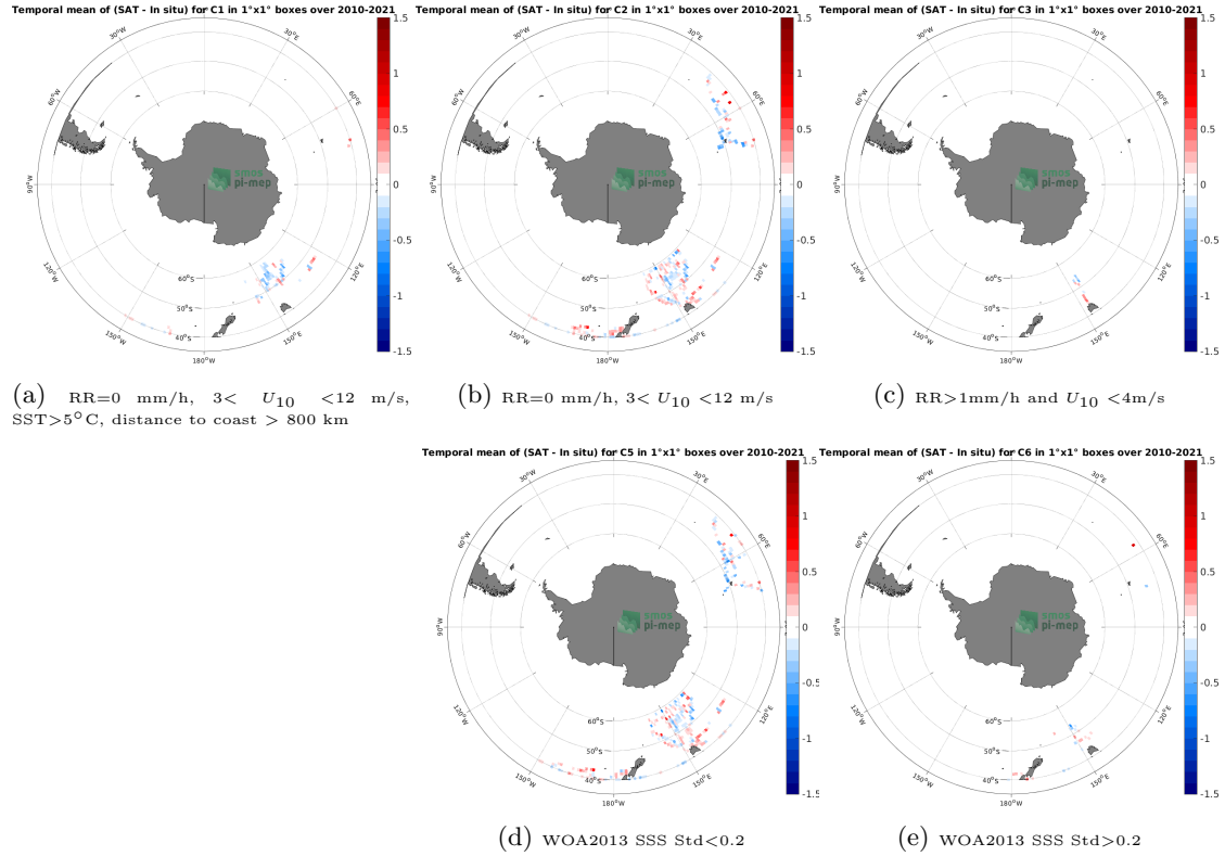
Figure 12: Temporal mean gridded over spatial boxes of size 1^{\circ}\times 1^{\circ} of \Delta\text{SSS} (SMOS SSS L3 v332 - 9 Days (CATDS-CPDC) - TSG (LEGOS-DM)) for 5 different subdatasets corresponding to:RR=0 mm/h, 3 < U_{10} < 12 m/s, SST >5^{\circ}\text{C} , distance to coast > 800 km (a), RR=0 mm/h, 3 < U_{10} < 12 m/s (b), RR >1 mm/h and U_{10} < 4 m/s (c), WOA2013 SSS Std <0.2 (d), WOA2013 SSS Std >0.2 (e).
