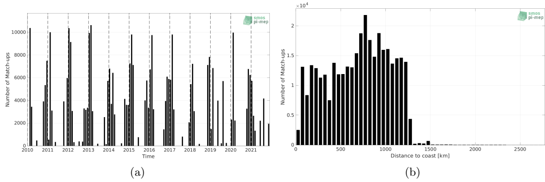
Figure 1: Number of match-ups between TSG (LEGOS-DM) and SMOS SSS L3 v332 - 9 Days (CATDS-CPDC) SSS as a function of time (a) and as function of the distance to coast (b) over the Roaring Forties and Furious Fifties Pi-MEP region and for the full satellite product period.
