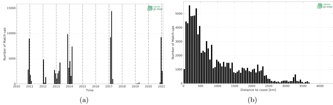
Figure 1: Number of match-ups between TSG (GOSUD-Sailing-ship) and SMOS SSS L3 v332 - 9 Days (CATDS-CPDC) SSS as a function of time (a) and as function of the distance to coast (b) over the Roaring Forties and Furious Fifties Pi-MEP region and for the full satellite product period.
