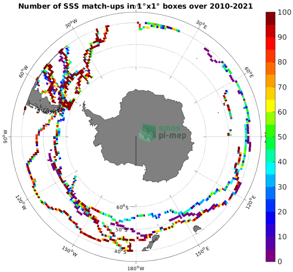
Figure 4: Number of SSS match-ups between TSG (GOSUD-Sailing-ship) SSS and the SMOS SSS L3 v332 - 9 Days (CATDS-CPDC) SSS product for the Roaring Forties and Furious Fifties Pi-MEP region over 1^{\circ} \times 1^{\circ} boxes and for the full satellite product period.
