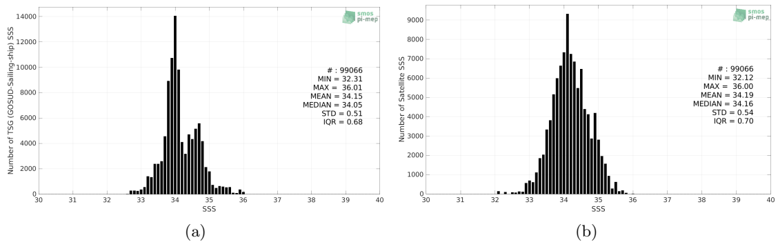
Figure 2: Histograms of SSS from TSG (GOSUD-Sailing-ship) (a) and SMOS SSS L3 v332 - 9 Days (CATDS-CPDC) (b) considering all match-up pairs per bins of 0.1 over the Roaring Forties and Furious Fifties Pi-MEP region and for the full satellite product period.
