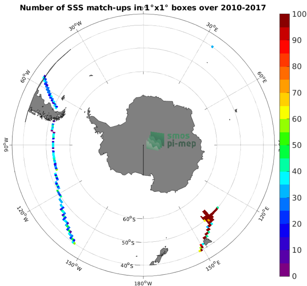
Figure 4: Number of SSS match-ups between TSG (GOSUD-Research-vessel) SSS and the SMOS SSS L3 v332 - 9 Days (CATDS-CPDC) SSS product for the Roaring Forties and Furious Fifties Pi-MEP region over 1^\circ \times 1^\circ boxes and for the full satellite product period.
