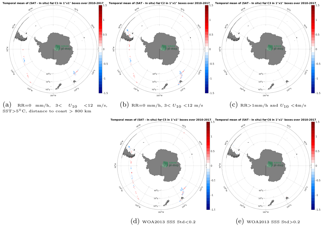
Figure 12: Temporal mean gridded over spatial boxes of size 1^{\circ} \times 1^{\circ} of \Delta SSS (SMOS SSS L3 v332 - 9 Days (CATDS-CPDC) - TSG (GOSUD-Research-vessel)) for 5 different subdatasets corresponding to:RR=0 mm/h, 3 < U_{10} < 12 m/s, SST>5°C, distance to coast > 800 km (a), RR=0 mm/h, 3 < U_{10} < 12 m/s (b), RR>1mm/h and U_{10} < 4 m/s (c), WOA2013 SSS Std<0.2 (d), WOA2013 SSS Std>0.2 (e).
