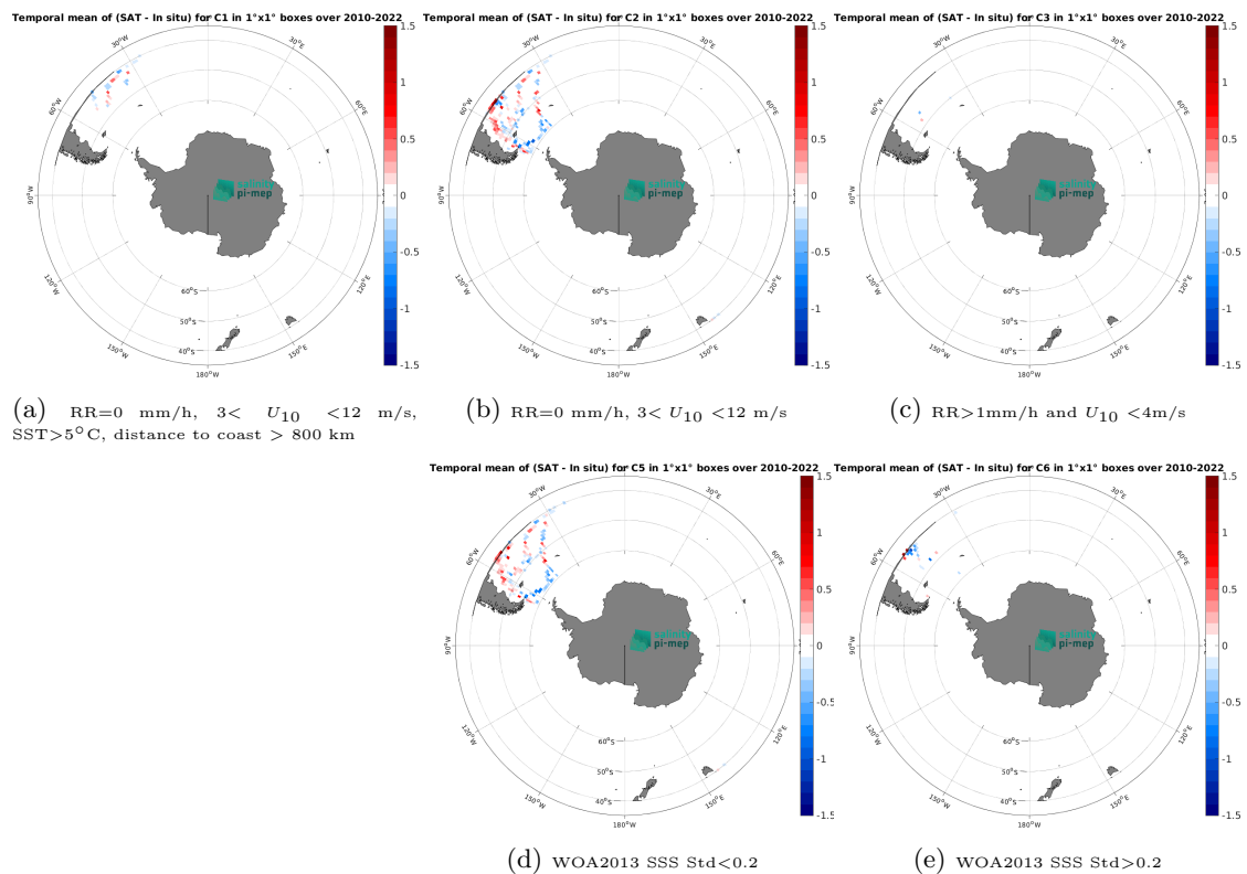
Figure 14: Temporal mean gridded over spatial boxes of size 1^\circ \times 1^\circ of \Delta\text{SSS} (SMOS SSS L3 v332 - 9 Days (CATDS-CPDC) - TSG (CSIC-UTM)) for 5 different subdatasets corresponding to: RR=0 mm/h, 3 < U_{10} < 12 m/s, SST > 5°C, distance to coast > 800 km (a), RR=0 mm/h, 3 < U_{10} < 12 m/s (b), RR > 1mm/h and U_{10} < 4 m/s (c), WOA2013 SSS Std < 0.2 (d), WOA2013 SSS Std > 0.2 (e).
