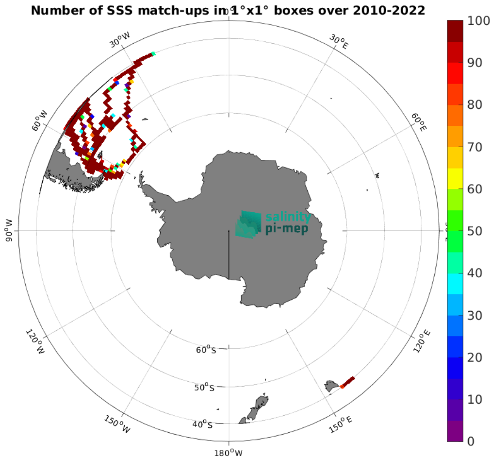
Figure 5: Number of SSS match-ups between TSG (CSIC-UTM) SSS and the SMOS SSS L3 v332 - 9 Days (CATDS-CPDC) SSS product for the Roaring Forties and Furious Fifties Pi-MEP region over 1^\circ \times 1^\circ boxes and for the full satellite product period.
