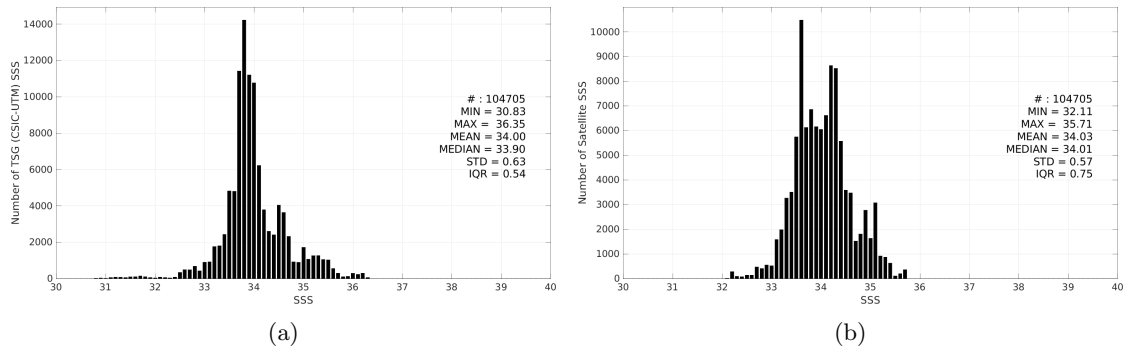
Figure 3: Histograms of SSS from TSG (CSIC-UTM) (a) and SMOS SSS L3 v332 - 9 Days (CATDS-CPDC) (b) considering all match-up pairs per bins of 0.1 over the Roaring Forties and Furious Fifties Pi-MEP region and for the full satellite product period.
