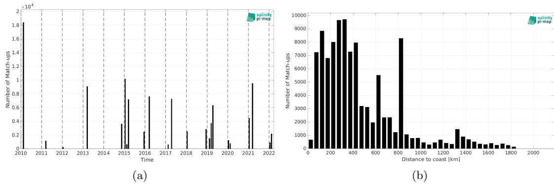
Figure 2: Number of match-ups between TSG (CSIC-UTM) and SMOS SSS L3 v332 - 9 Days (CATDS-CPDC) SSS as a function of time (a) and as function of the distance to coast (b) over the Roaring Forties and Furious Fifties Pi-MEP region and for the full satellite product period.
