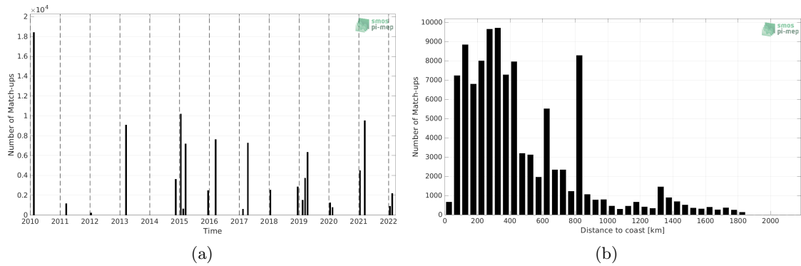
Figure 1: Number of match-ups between TSG (CSIC-UTM) and SMOS SSS L3 v332 - 9 Days (CATDS-CPDC) SSS as a function of time (a) and as function of the distance to coast (b) over the Roaring Forties and Furious Fifties Pi-MEP region and for the full satellite product period.
