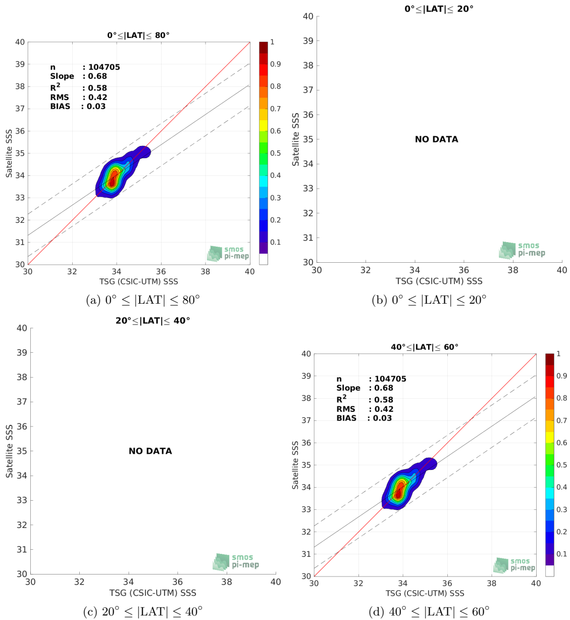
Figure 9: Contour maps of the concentration of SMOS SSS L3 v332 - 9 Days (CATDS-CPDC) SSS (y-axis) versus TSG (CSIC-UTM) SSS (x-axis) at match-up pairs for different latitude bands. For each plot, the red line shows x=y . The black thin and dashed lines indicate a linear fit through the data cloud and the \pm 95\% confidence levels, respectively. The number match-up pairs n , the slope and R^2 coefficient of the linear fit, the root mean square (RMS) and the mean bias between satellite and in situ data are indicated for each latitude band in each plots.
