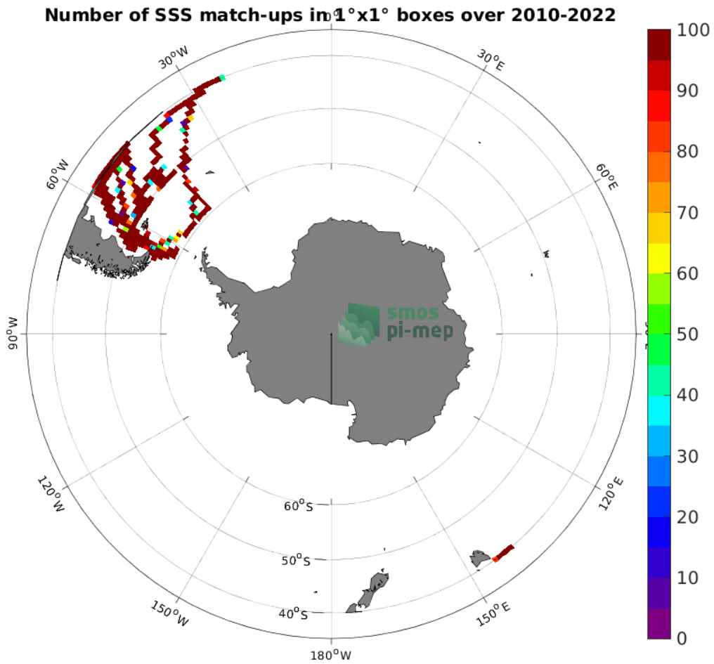
Figure 4: Number of SSS match-ups between TSG (CSIC-UTM) SSS and the SMOS SSS L3 v332 - 9 Days (CATDS-CPDC) SSS product for the Roaring Forties and Furious Fifties Pi-MEP region over 1^\circ \times 1^\circ boxes and for the full satellite product period.
