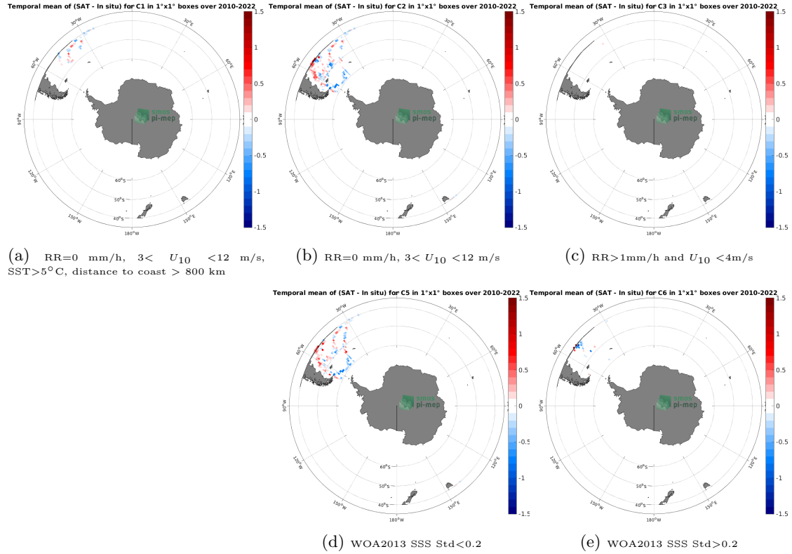
Figure 12: Temporal mean gridded over spatial boxes of size 1^{\circ}\times 1^{\circ} of \Delta\text{SSS} (SMOS SSS L3 v332 - 9 Days (CATDS-CPDC) - TSG (CSIC-UTM)) for 5 different subdatasets corresponding to:RR=0 mm/h, 3 < U_{10} < 12 m/s, SST >5^{\circ}\text{C} , distance to coast > 800 km (a), RR=0 mm/h, 3 < U_{10} < 12 m/s (b), RR >1 mm/h and U_{10} < 4 m/s (c), WOA2013 SSS Std <0.2 (d), WOA2013 SSS Std >0.2 (e).
