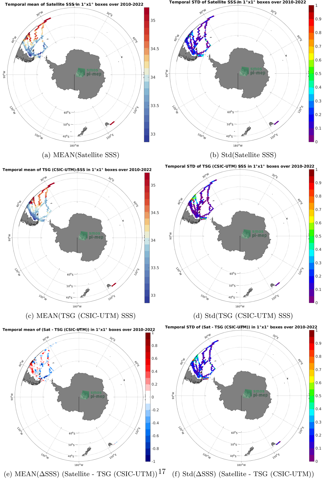
Figure 6: Temporal mean (left) and Std (right) of SSS from SMOS SSS L3 v332 - 9 Days (CATDS-CPDC) (top), TSG (CSIC-UTM) (middle), and of \Delta SSS (Satellite - TSG (CSIC-UTM)). Only match-up pairs are used to generate these maps.
