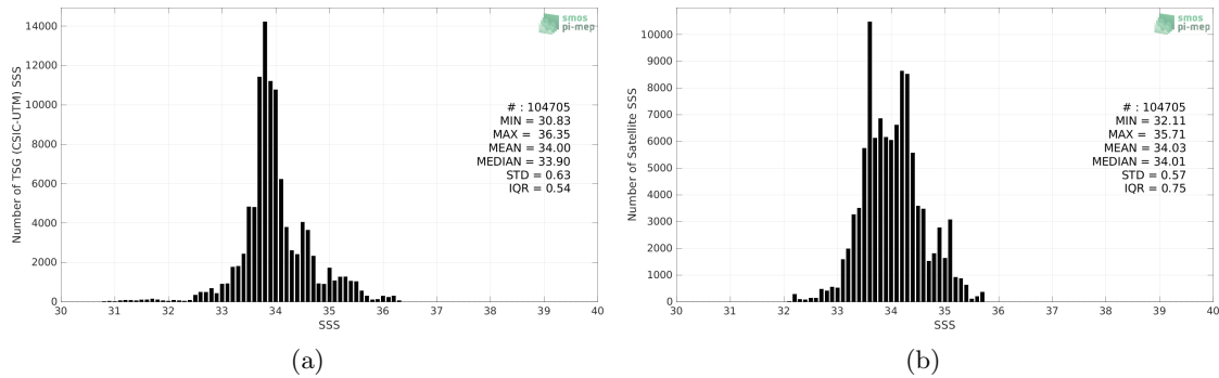
Figure 2: Histograms of SSS from TSG (CSIC-UTM) (a) and SMOS SSS L3 v332 - 9 Days (CATDS-CPDC) (b) considering all match-up pairs per bins of 0.1 over the Roaring Forties and Furious Fifties Pi-MEP region and for the full satellite product period.
