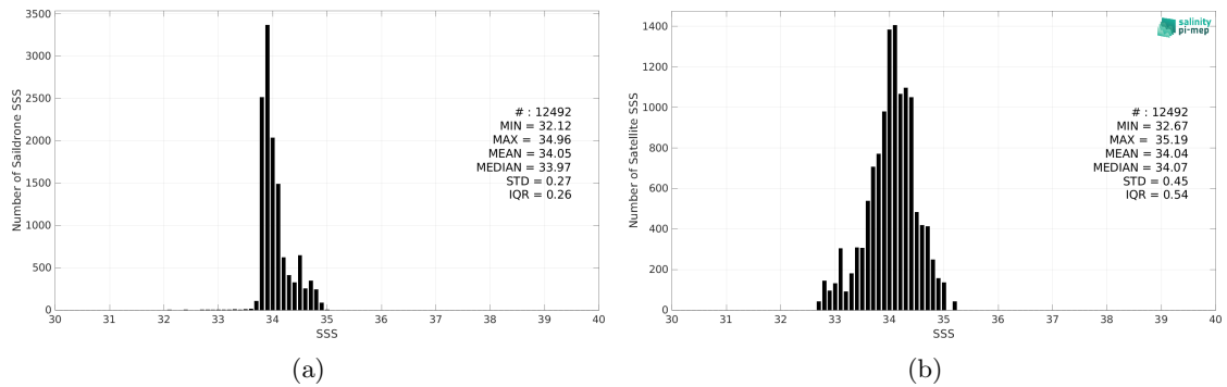
Figure 2: Histograms of SSS from Saildrone (a) and SMOS SSS L3 v332 - 9 Days (CATDS-CPDC) (b) considering all match-up pairs per bins of 0.1 over the Roaring Forties and Furious Fifties Pi-MEP region and for the full satellite product period.
