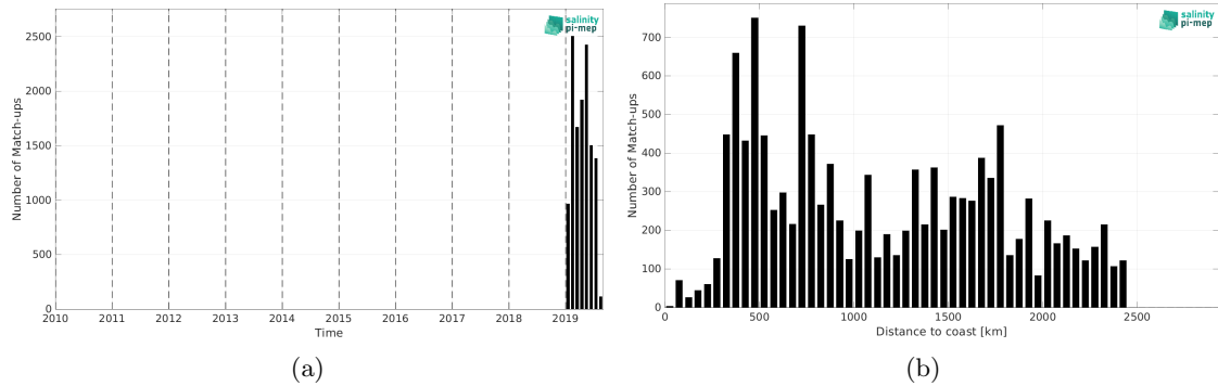
Figure 1: Number of match-ups between Saildrone and SMOS SSS L3 v332 - 9 Days (CATDS-CPDC) SSS as a function of time (a) and as function of the distance to coast (b) over the Roaring Forties and Furious Fifties Pi-MEP region and for the full satellite product period.
