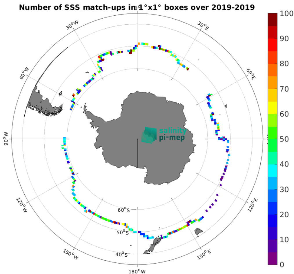
Figure 4: Number of SSS match-ups between Saildrone SSS and the SMOS SSS L3 v332 - 9 Days (CATDS-CPDC) SSS product for the Roaring Forties and Furious Fifties Pi-MEP region over 1^\circ \times 1^\circ boxes and for the full satellite product period.
