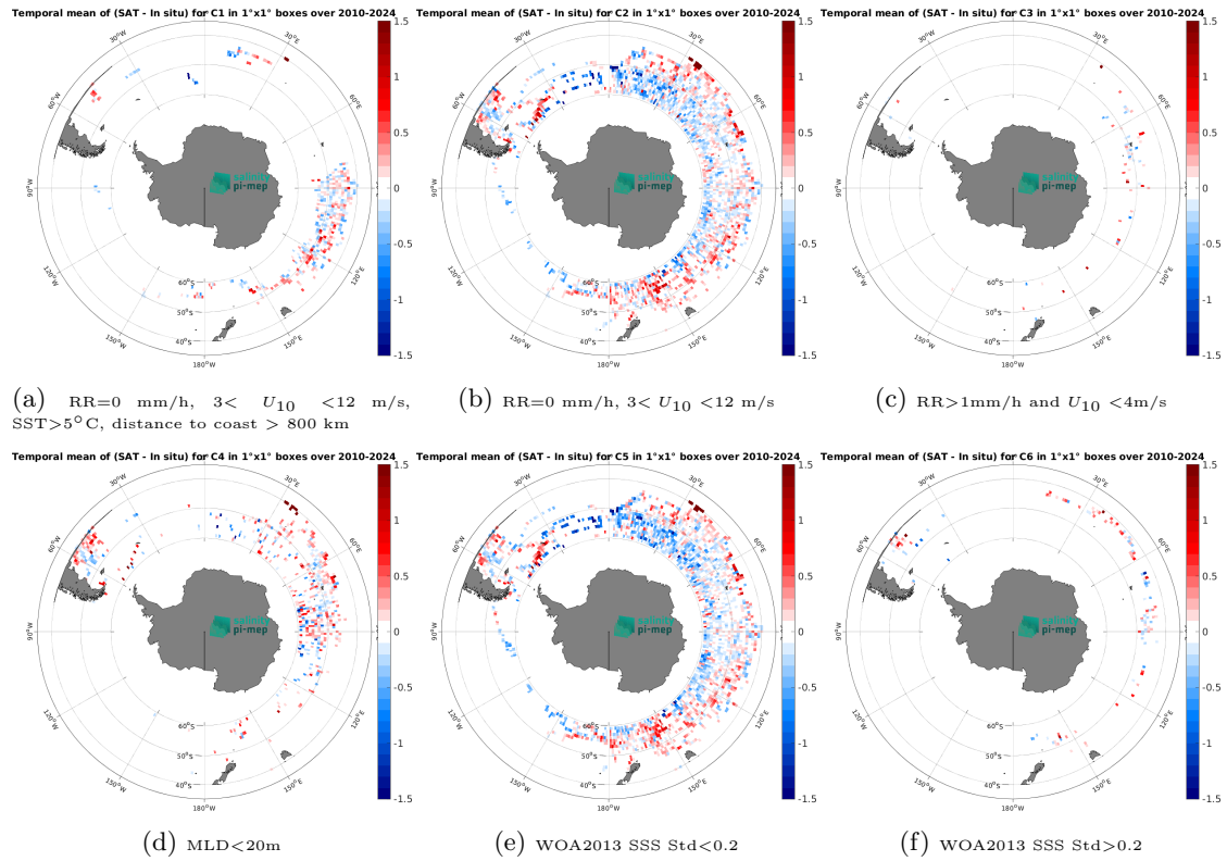
Figure 14: Temporal mean gridded over spatial boxes of size 1^\circ \times 1^\circ of \Delta\text{SSS} (SMOS SSS L3 v332 - 9 Days (CATDS-CPDC) - Marine mammals) for 6 different subdatasets corresponding to: RR=0 mm/h, 3 < U_{10} < 12 m/s, SST>5°C, distance to coast > 800 km (a), RR=0 mm/h, 3 < U_{10} < 12 m/s (b), RR>1mm/h and U_{10} < 4 m/s (c),MLD<20m (d),WOA2013 SSS Std<0.2 (e),WOA2013 SSS Std>0.2 (f).
