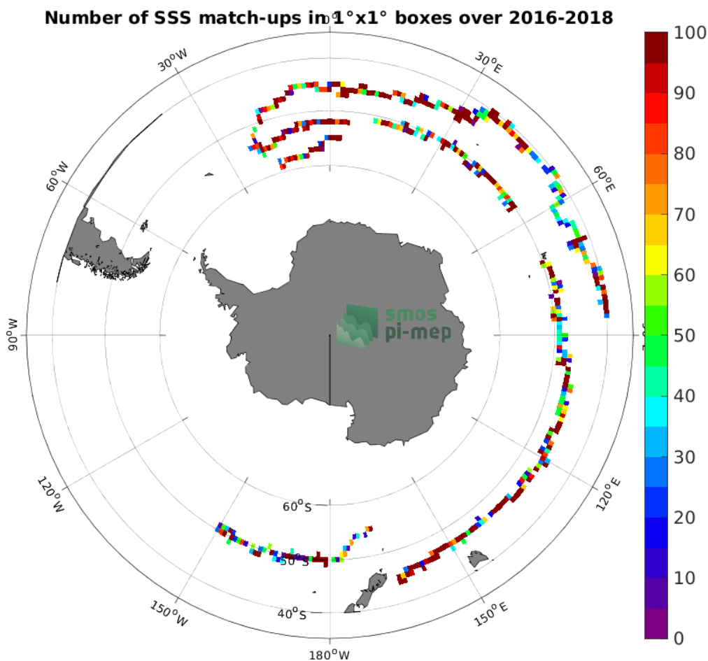
Figure 3: Number of SSS match-ups between Surface drifters SSS and the SMOS SSS L3 v332 - 9 Days (CATDS-CPDC) SSS product for the Roaring Forties and Furious Fifties Pi-MEP region over 1^\circ \times 1^\circ boxes and for the full satellite product period.
