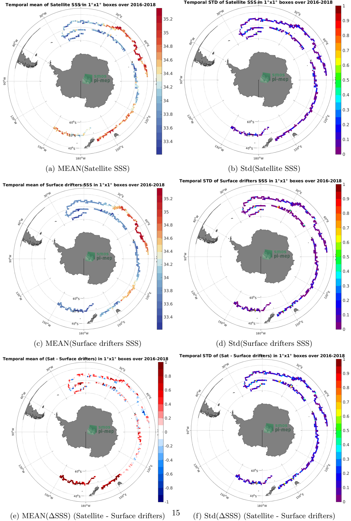
Figure 5: Temporal mean (left) and Std (right) of SSS from SMOS SSS L3 v332 - 9 Days (CATDS-CPDC) (top), Surface drifters (middle), and of \Delta SSS (Satellite - Surface drifters). Only match-up pairs are used to generate these maps.
