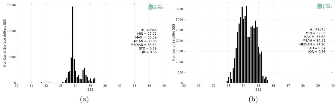
Figure 2: Histograms of SSS from Surface drifters (a) and SMOS SSS L3 v332 - 9 Days (CATDS-CPDC) (b) considering all match-up pairs per bins of 0.1 over the Roaring Forties and Furious Fifties Pi-MEP region and for the full satellite product period.
