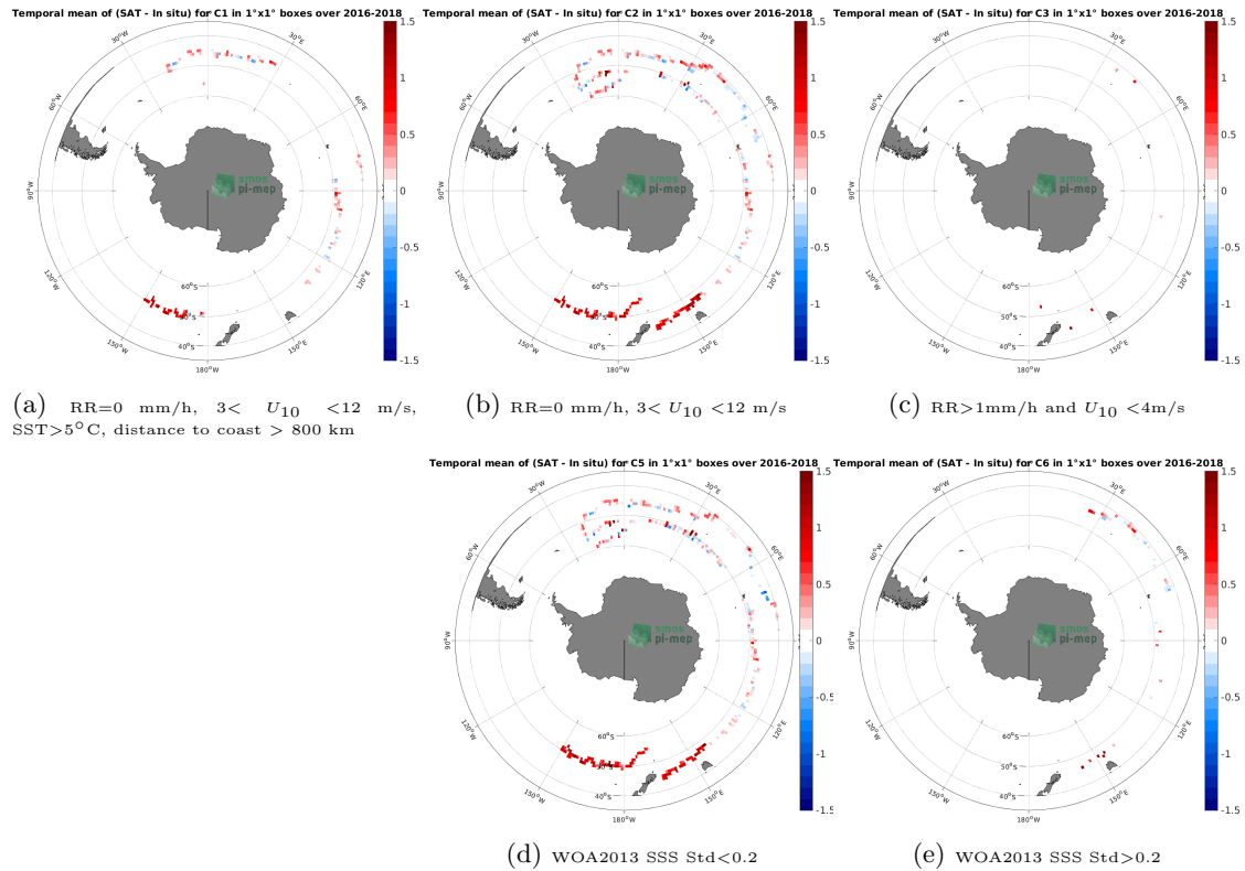
Figure 11: Temporal mean gridded over spatial boxes of size 1^{\circ}\times 1^{\circ} of \Delta\text{SSS} (SMOS SSS L3 v332 - 9 Days (CATDS-CPDC) - Surface drifters) for 5 different subdatasets corresponding to:RR=0 mm/h, 3 < U_{10} < 12 m/s, SST >5^{\circ}\text{C} , distance to coast > 800 km (a), RR=0 mm/h, 3 < U_{10} < 12 m/s (b), RR >1 mm/h and U_{10} < 4 m/s (c), WOA2013 SSS Std <0.2 (d), WOA2013 SSS Std >0.2 (e).
