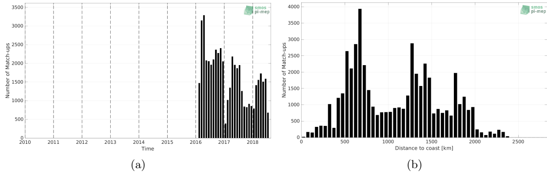
Figure 1: Number of match-ups between Surface drifters and SMOS SSS L3 v332 - 9 Days (CATDS-CPDC) SSS as a function of time (a) and as function of the distance to coast (b) over the Roaring Forties and Furious Fifties Pi-MEP region and for the full satellite product period.
