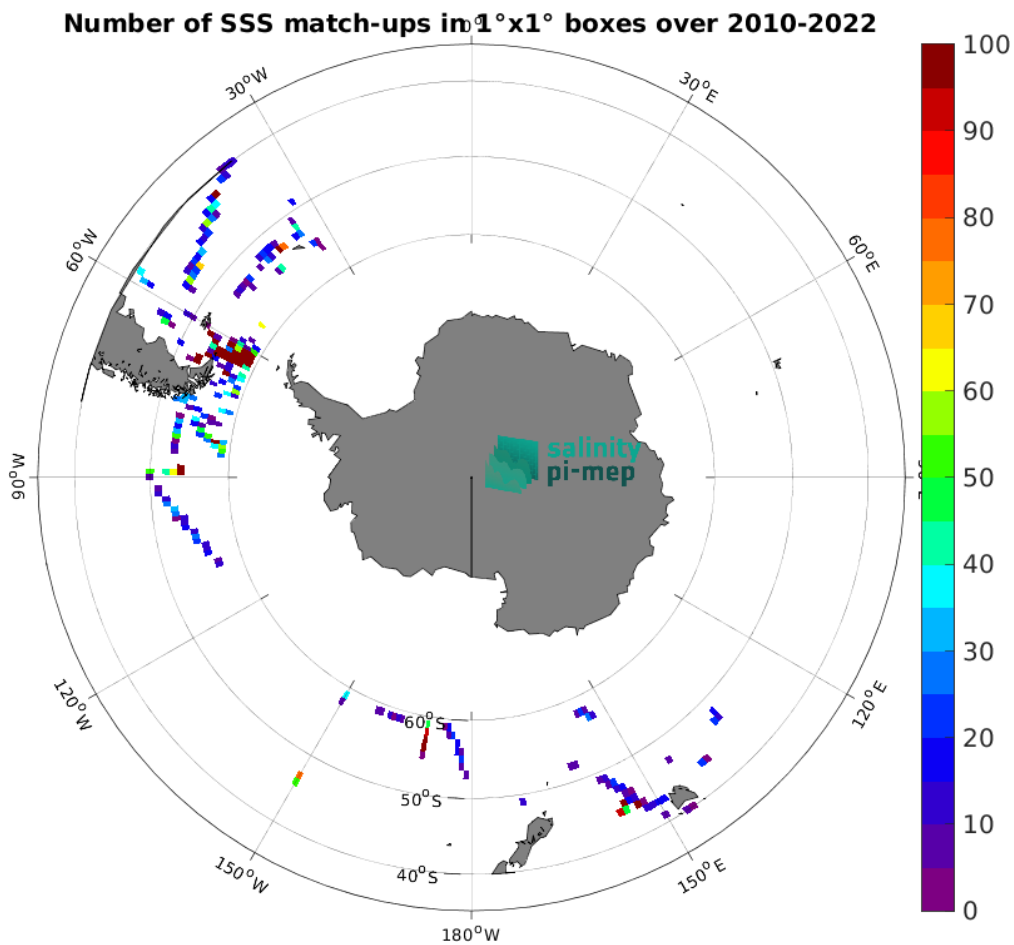
Figure 4: Number of SSS match-ups between TSG (SAMOS) SSS and the SMOS SSS L2Q v331 - 0.25 Deg (CATDS-CPDC) SSS product for the Roaring Forties and Furious Fifties Pi-MEP region over 1^{\circ} \times 1^{\circ} boxes and for the full satellite product period.
