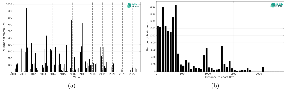
Figure 1: Number of match-ups between TSG (SAMOS) and SMOS SSS L2Q v331 - 0.25 Deg (CATDS-CPDC) SSS as a function of time (a) and as function of the distance to coast (b) over the Roaring Forties and Furious Fifties Pi-MEP region and for the full satellite product period.
