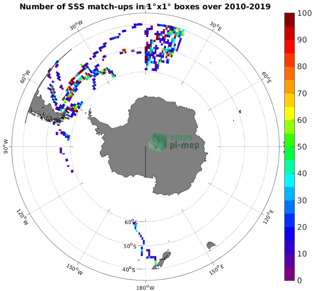
Figure 4: Number of SSS match-ups between TSG (Polarstern) SSS and the SMOS SSS L2Q v331 - 0.25 Deg (CATDS-CPDC) SSS product for the Roaring Forties and Furious Fifties Pi-MEP region over 1^\circ \times 1^\circ boxes and for the full satellite product period.
