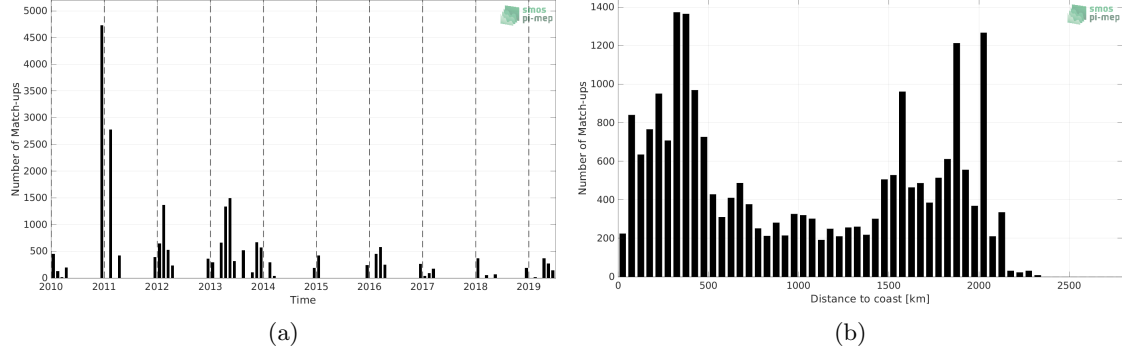
Figure 1: Number of match-ups between TSG (Polarstern) and SMOS SSS L2Q v331 - 0.25 Deg (CATDS-CPDC) SSS as a function of time (a) and as function of the distance to coast (b) over the Roaring Forties and Furious Fifties Pi-MEP region and for the full satellite product period.
