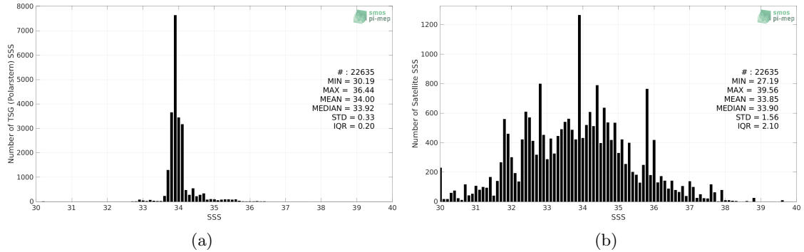
Figure 2: Histograms of SSS from TSG (Polarstern) (a) and SMOS SSS L2Q v331 - 0.25 Deg (CATDS-CPDC) (b) considering all match-up pairs per bins of 0.1 over the Roaring Forties and Furious Fifties Pi-MEP region and for the full satellite product period.
