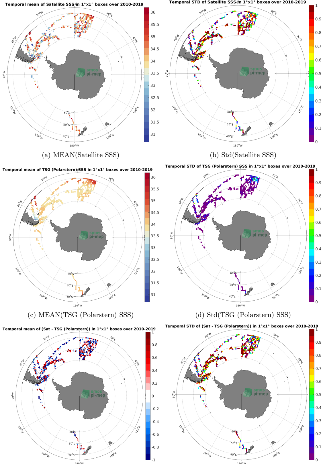
(e) MEAN( \Delta SSS) (Satellite - TSG (Polarstern)) 16 (f) Std( \Delta SSS) (Satellite - TSG (Polarstern)) Figure 6: Temporal mean (left) and Std (right) of SSS from SMOS SSS L2Q v331 - 0.25 Deg (CATDS-CPDC) (top), TSG (Polarstern) (middle), and of \Delta SSS (Satellite - TSG (Polarstern)). Only match-up pairs are used to generate these maps.
