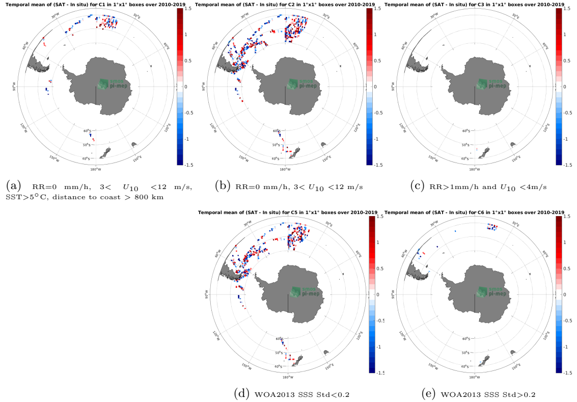
Figure 12: Temporal mean gridded over spatial boxes of size 1^{\circ}\times 1^{\circ} of \Delta\text{SSS} (SMOS SSS L2Q v331 - 0.25 Deg (CATDS-CPDC) - TSG (Polarstern)) for 5 different subdatasets corresponding to:RR=0 mm/h, 3 < U_{10} < 12 m/s, SST >5^{\circ}\text{C} , distance to coast > 800 km (a), RR=0 mm/h, 3 < U_{10} < 12 m/s (b), RR >1 mm/h and U_{10} < 4 m/s (c), WOA2013 SSS Std <0.2 (d), WOA2013 SSS Std >0.2 (e).
