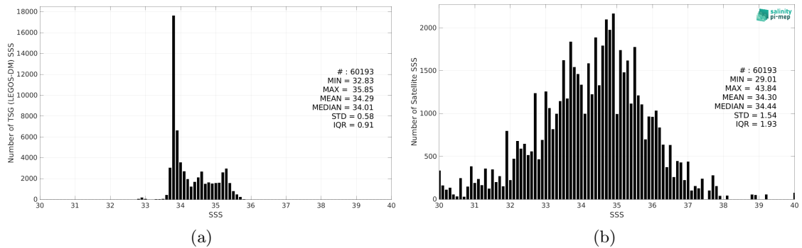
Figure 2: Histograms of SSS from TSG (LEGOS-DM) (a) and SMOS SSS L2Q v331 - 0.25 Deg (CATDS-CPDC) (b) considering all match-up pairs per bins of 0.1 over the Roaring Forties and Furious Fifties Pi-MEP region and for the full satellite product period.
