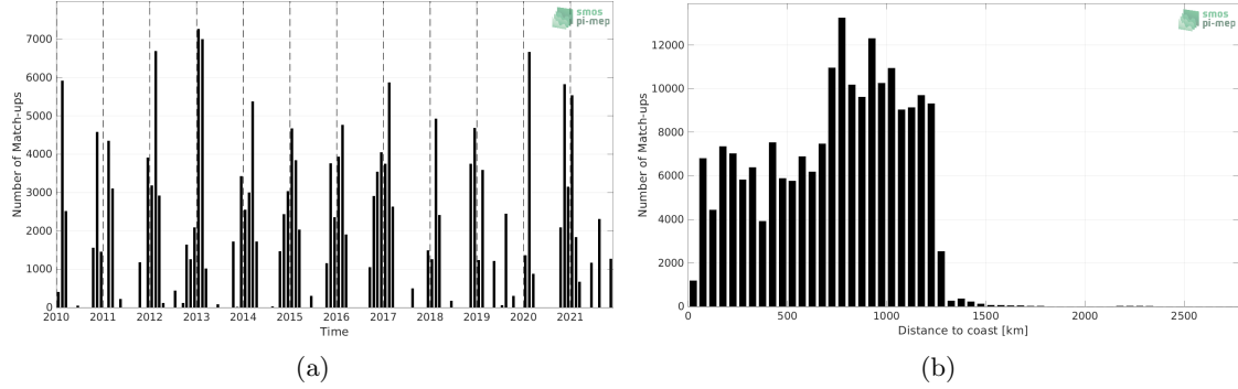
Figure 1: Number of match-ups between TSG (LEGOS-DM) and SMOS SSS L2Q v331 - 0.25 Deg (CATDS-CPDC) SSS as a function of time (a) and as function of the distance to coast (b) over the Roaring Forties and Furious Fifties Pi-MEP region and for the full satellite product period.
