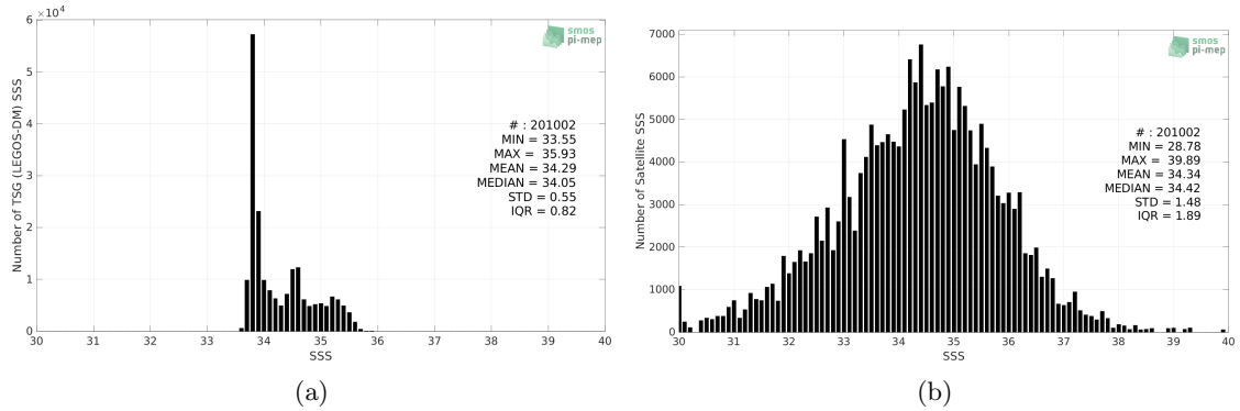
Figure 2: Histograms of SSS from TSG (LEGOS-DM) (a) and SMOS SSS L2Q v331 - 0.25 Deg (CATDS-CPDC) (b) considering all match-up pairs per bins of 0.1 over the Roaring Forties and Furious Fifties Pi-MEP region and for the full satellite product period.
