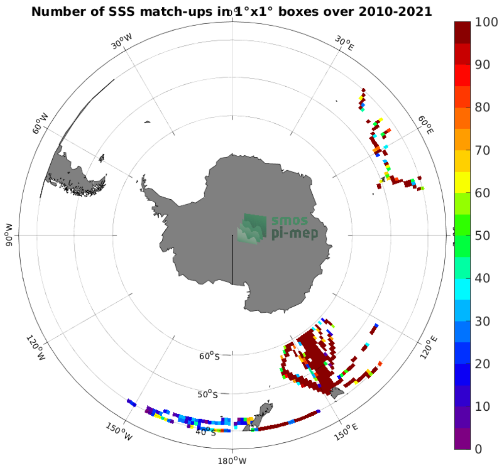
Figure 4: Number of SSS match-ups between TSG (LEGOS-DM) SSS and the SMOS SSS L2Q v331 - 0.25 Deg (CATDS-CPDC) SSS product for the Roaring Forties and Furious Fifties Pi-MEP region over 1^\circ \times 1^\circ boxes and for the full satellite product period.
