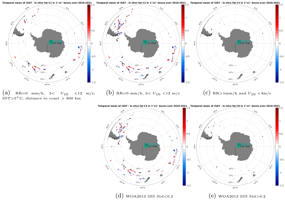
Figure 12: Temporal mean gridded over spatial boxes of size 1°×1° of \Delta SSS (SMOS SSS L2Q v331 - 0.25 Deg (CATDS-CPDC) - TSG (GOSUD-Sailing-ship)) for 5 different subdatasets corresponding to:RR=0 mm/h, 3 < U_{10} < 12 m/s, SST>5°C, distance to coast > 800 km (a), RR=0 mm/h, 3 < U_{10} < 12 m/s (b), RR>1mm/h and U_{10} < 4 m/s (c), WOA2013 SSS Std<0.2 (d), WOA2013 SSS Std>0.2 (e).
