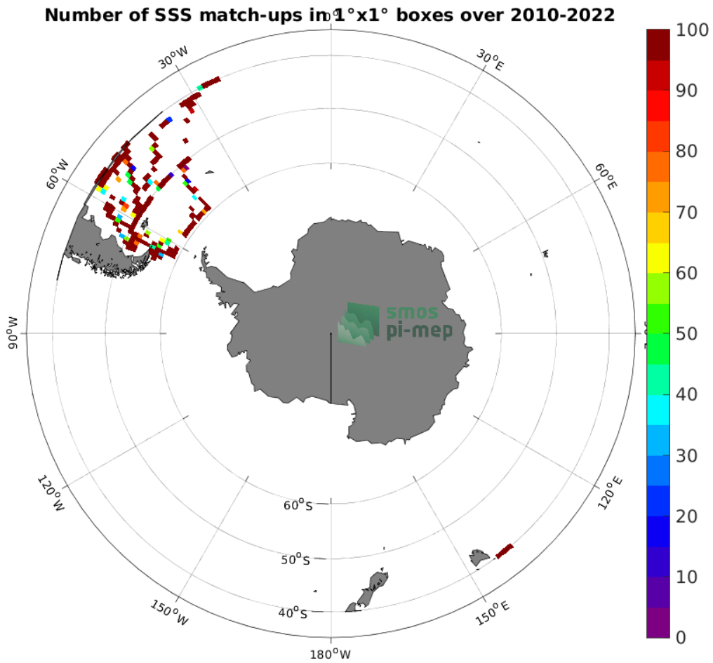
Figure 4: Number of SSS match-ups between TSG (CSIC-UTM) SSS and the SMOS SSS L2Q v331 - 0.25 Deg (CATDS-CPDC) SSS product for the Roaring Forties and Furious Fifties Pi-MEP region over 1^\circ \times 1^\circ boxes and for the full satellite product period.
