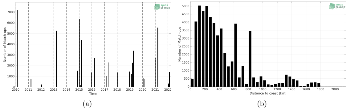
Figure 1: Number of match-ups between TSG (CSIC-UTM) and SMOS SSS L2Q v331 - 0.25 Deg (CATDS-CPDC) SSS as a function of time (a) and as function of the distance to coast (b) over the Roaring Forties and Furious Fifties Pi-MEP region and for the full satellite product period.
