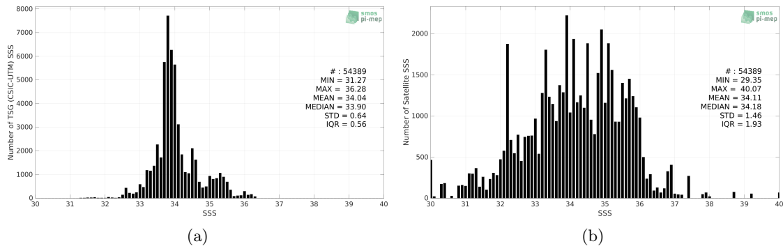
Figure 2: Histograms of SSS from TSG (CSIC-UTM) (a) and SMOS SSS L2Q v331 - 0.25 Deg (CATDS-CPDC) (b) considering all match-up pairs per bins of 0.1 over the Roaring Forties and Furious Fifties Pi-MEP region and for the full satellite product period.
