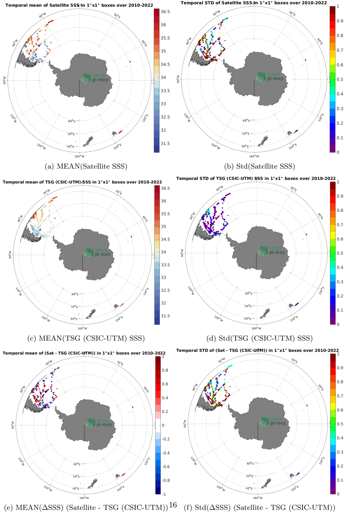
Figure 6: Temporal mean (left) and Std (right) of SSS from SMOS SSS L2Q v331 - 0.25 Deg (CATDS-CPDC) (top), TSG (CSIC-UTM) (middle), and of \Delta SSS (Satellite - TSG (CSIC-UTM)). Only match-up pairs are used to generate these maps.
