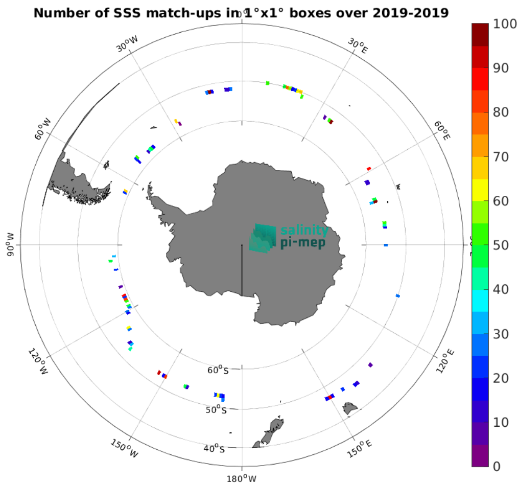
Figure 4: Number of SSS match-ups between Saildrone SSS and the SMOS SSS L2Q v331 - 0.25 Deg (CATDS-CPDC) SSS product for the Roaring Forties and Furious Fifties Pi-MEP region over 1^{\circ} \times 1^{\circ} boxes and for the full satellite product period.
